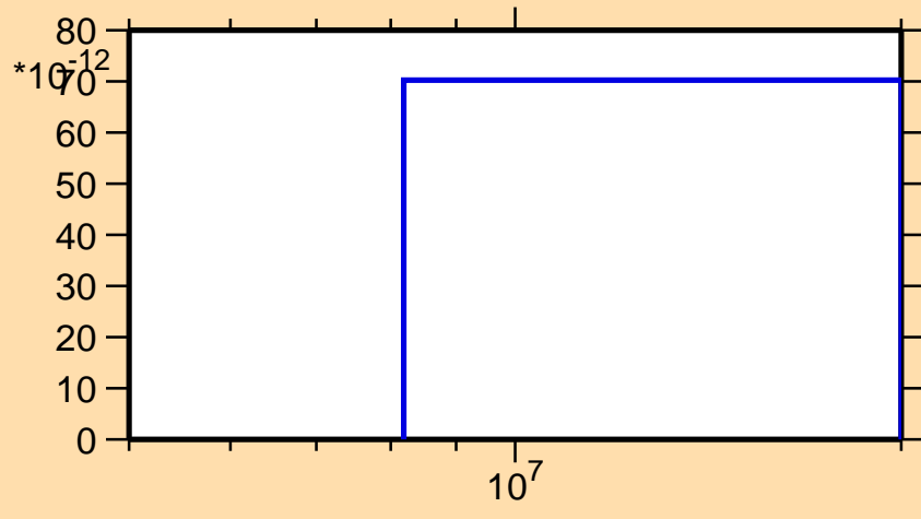
\sigma vs. E for ^{211}\text{Rn}(\text{mt } 45)
