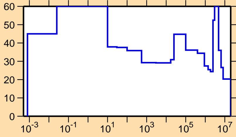
\Delta\sigma/\sigma vs. E for ^{211}\text{Rn}(n,p)
