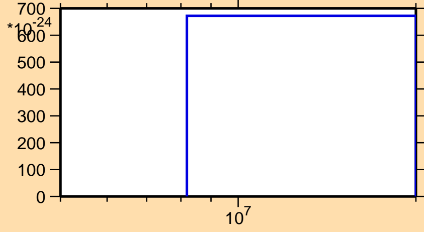
\sigma vs. E for ^{211}\text{Rn} (mt 42)
