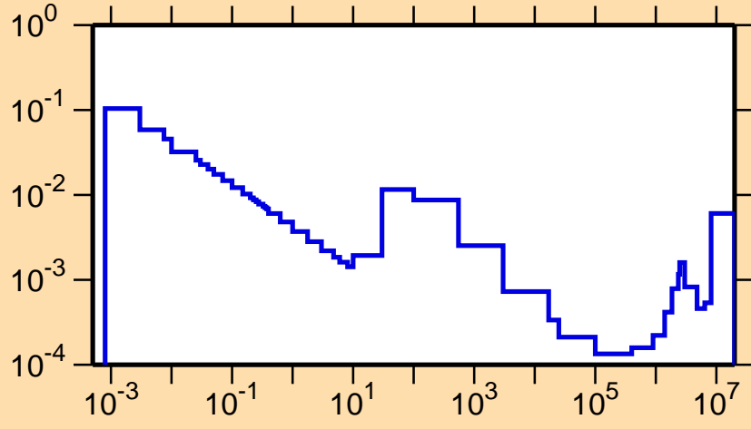
\sigma vs. E for ^{211}\text{Rn}(n,\alpha)
