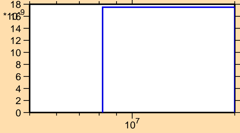
\sigma vs. E for ^{211}\text{Rn}(n,3n\alpha)
