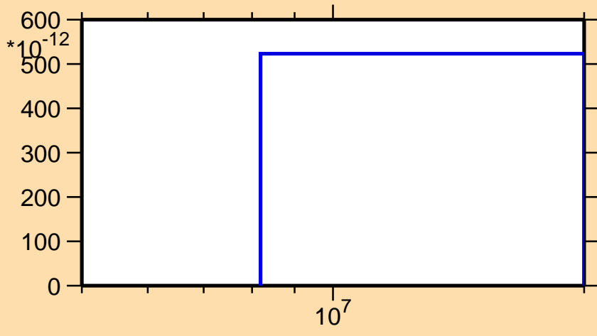
\sigma vs. E for ^{211}\text{Rn}(n,nt)
