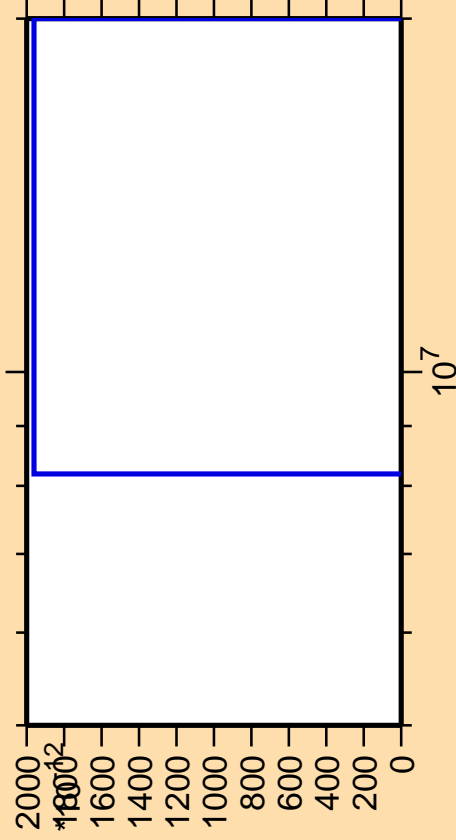
\Delta\sigma/\sigma vs. E for ^{211}\text{Rn} (mt 42)
