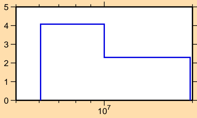
\Delta\sigma/\sigma vs. E for ^{212}\text{Rn}(n,2n)
