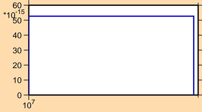
\sigma vs. E for ^{212}\text{Rn} (mt 34)
