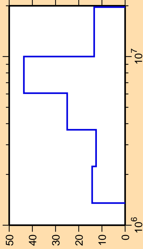
\Delta\sigma/\sigma vs. E for ^{212}\text{Rn}(n,n_4)
