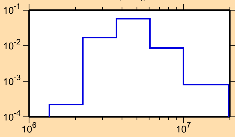
\sigma vs. E for ^{212}\text{Rn}(n,n_4)
