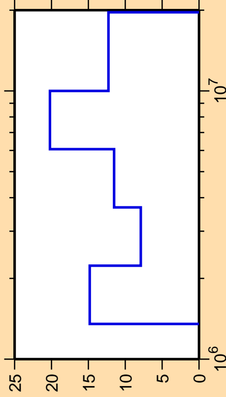
\Delta\sigma/\sigma vs. E for ^{212}\text{Rn}(n,n_2)
