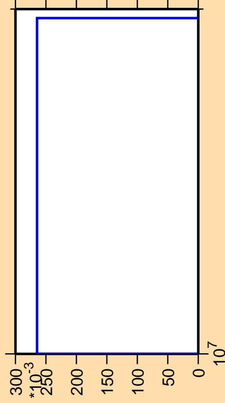
\Delta\sigma/\sigma vs. E for ^{212}\text{Rn} (mt 34)
