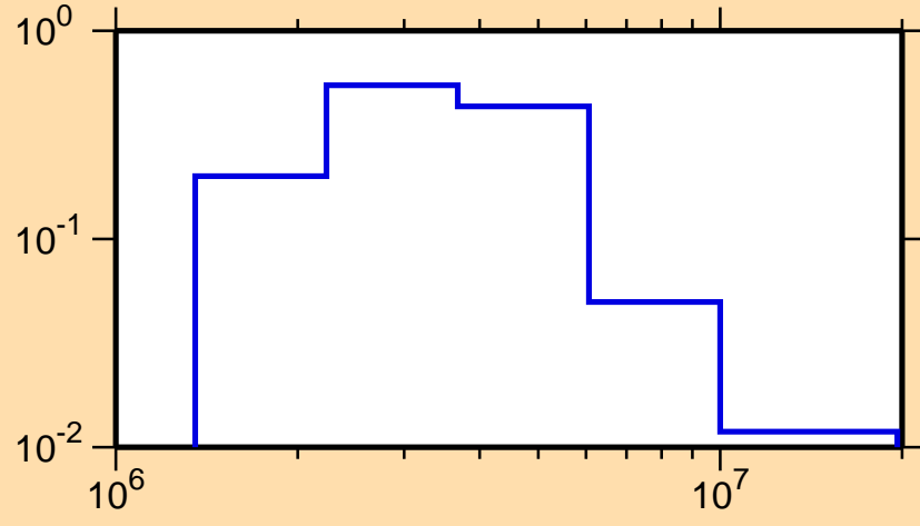
\sigma vs. E for ^{212}\text{Rn}(n,n_2)
