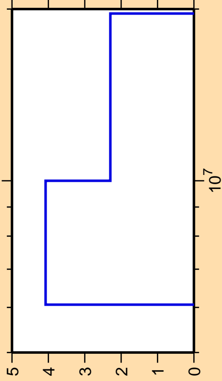
\Delta\sigma/\sigma vs. E for ^{212}\text{Rn}(n,2n)
