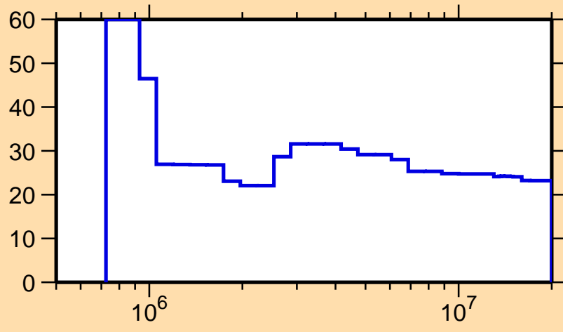
\Delta\sigma/\sigma vs. E for ^{219}\text{Rn}(n,\text{nonel.})
