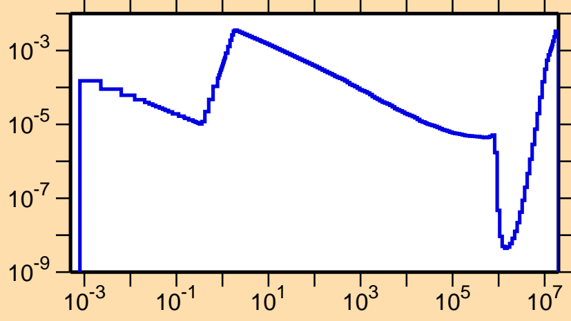
\sigma vs. E for ^{219}\text{Rn}(n,\alpha)
