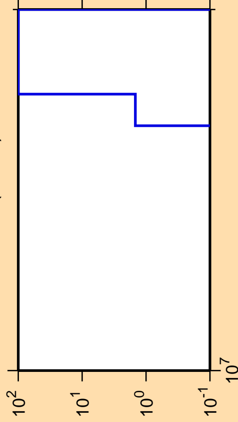
\Delta\sigma/\sigma vs. E for ^{219}\text{Rn} (mt 34)
