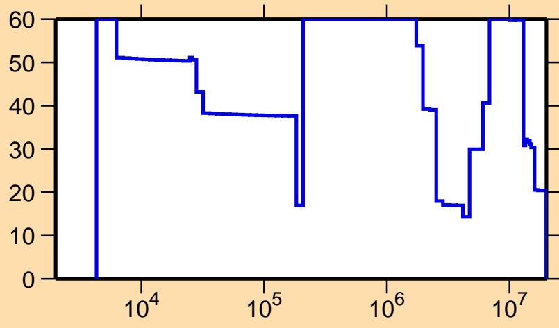
\Delta\sigma/\sigma vs. E for ^{219}\text{Rn}(n,\text{el.})
