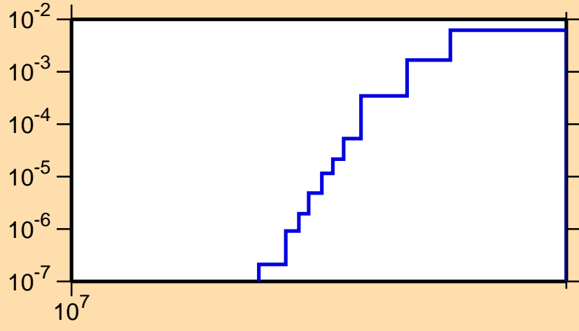
\sigma vs. E for ^{219}\text{Rn}(n,\text{nd})
