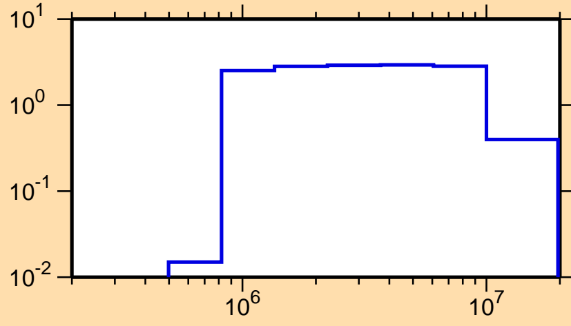
\sigma vs. E for ^{219}\text{Rn}(n,n\text{cont.})
