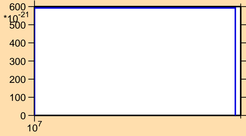
\sigma vs. E for ^{219}\text{Rn} (mt 11)
