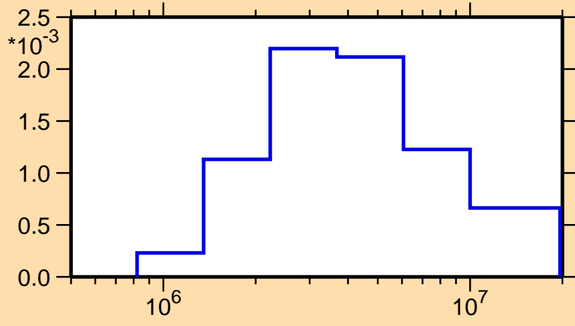
\sigma vs. E for ^{219}\text{Rn}(n,n\alpha)
