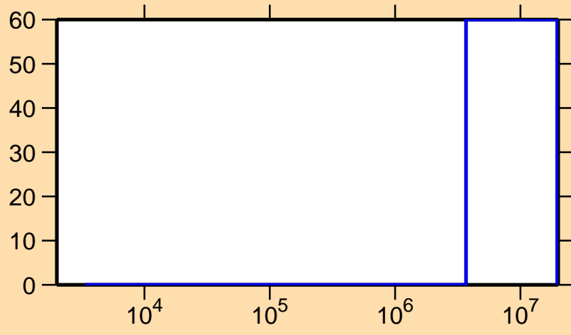
\Delta\sigma/\sigma vs. E for ^{219}\text{Rn}(n,f)
