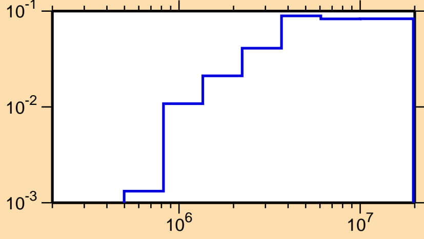
\sigma vs. E for ^{220}\text{Rn}(n,n_4)
