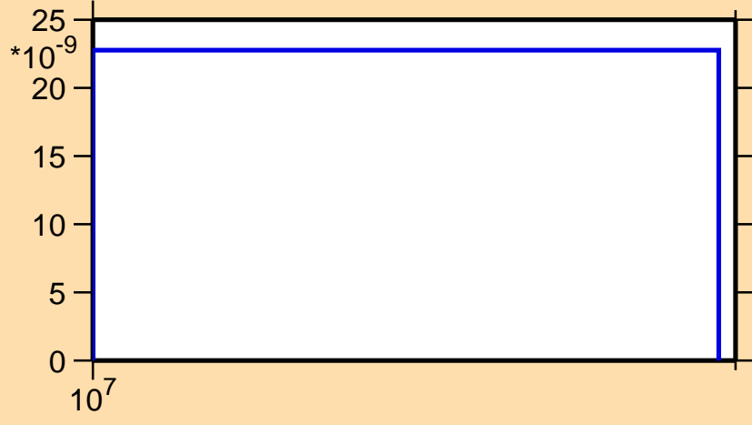
\sigma vs. E for ^{220}\text{Rn} (mt 45)
