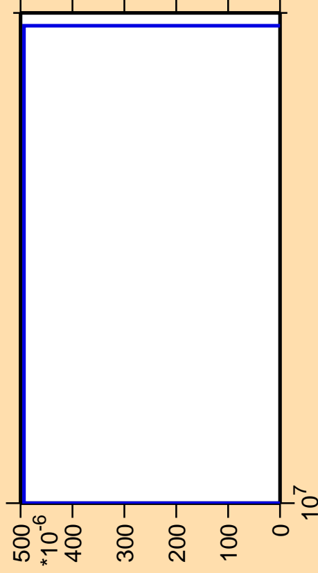
\Delta\sigma/\sigma vs. E for ^{220}\text{Rn} (mt 11)
