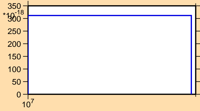
\sigma vs. E for ^{220}\text{Rn} (mt 11)
