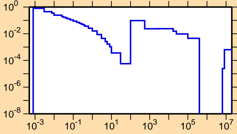
\sigma vs. E for ^{220}\text{Rn}(n,\gamma)
