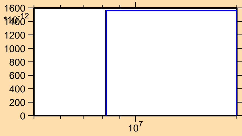
\sigma vs. E for ^{220}\text{Rn}(n,2np)
