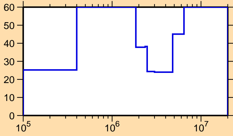
\Delta\sigma/\sigma vs. E for ^{220}\text{Rn}(n,\text{el.})
