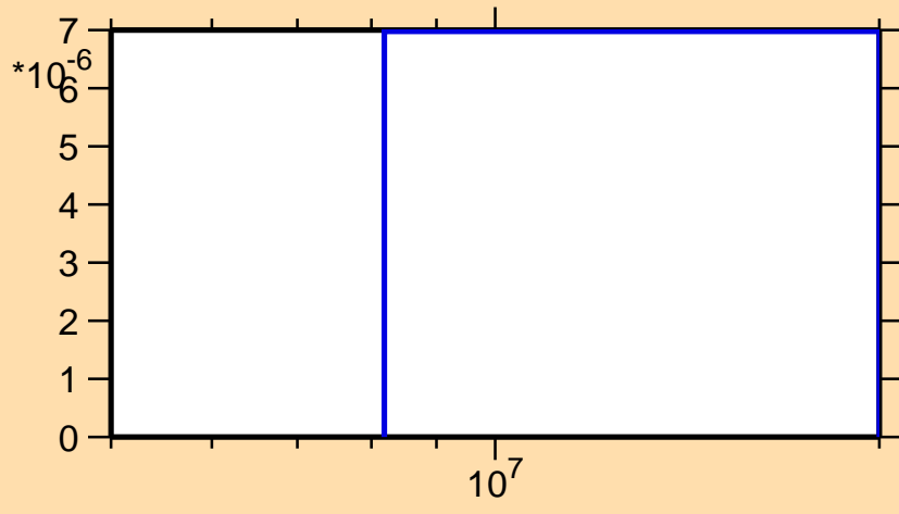
\sigma vs. E for ^{220}\text{Rn}(n,np)
