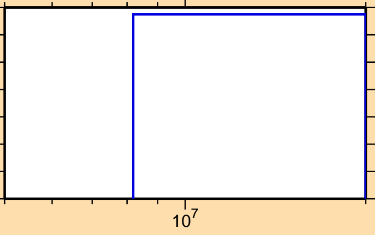
\sigma vs. E for ^{220}\text{Rn}(n,p\alpha)
