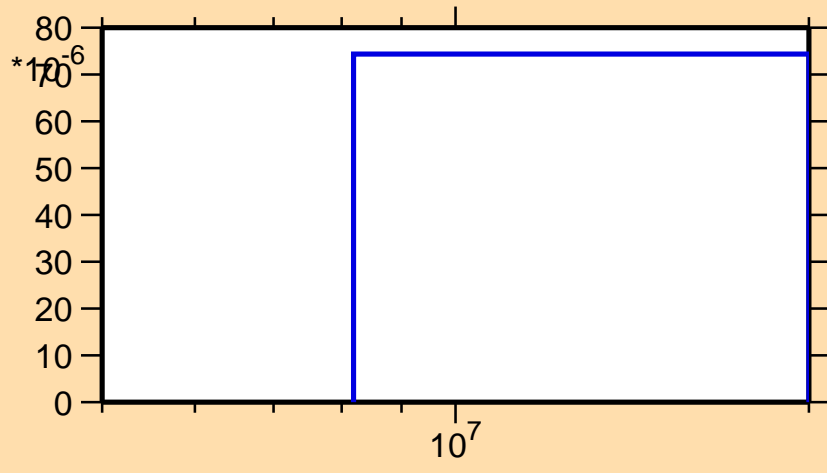
\sigma vs. E for ^{220}\text{Rn}(n,t)
