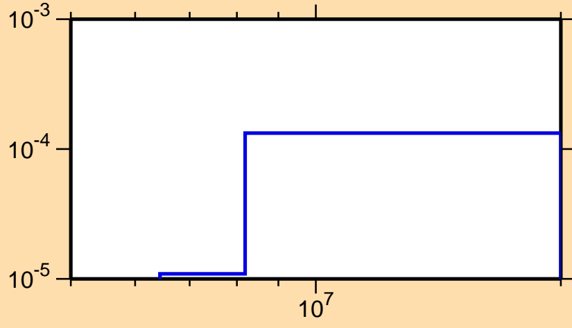
\sigma vs. E for ^{220}\text{Rn}(n,2n\alpha)
