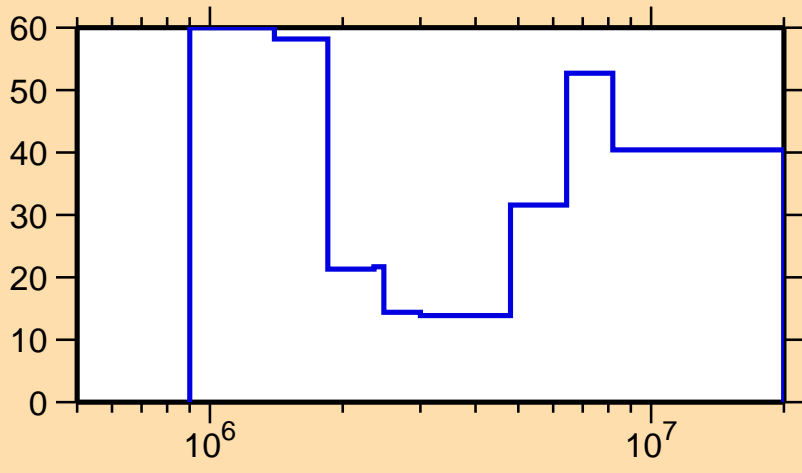
\Delta\sigma/\sigma vs. E for ^{220}\text{Rn}(n,\text{tot.})
