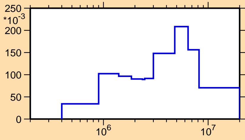
\sigma vs. E for ^{220}\text{Rn}(n,n_2)
