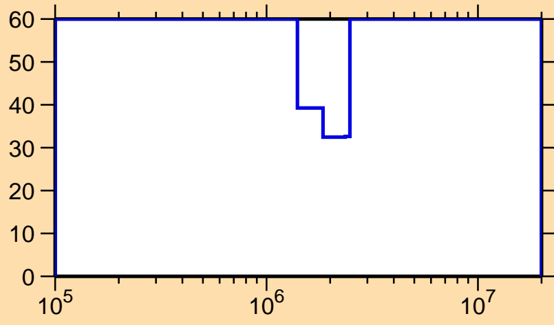
\Delta\sigma/\sigma vs. E for ^{220}\text{Rn}(n,n_1)
