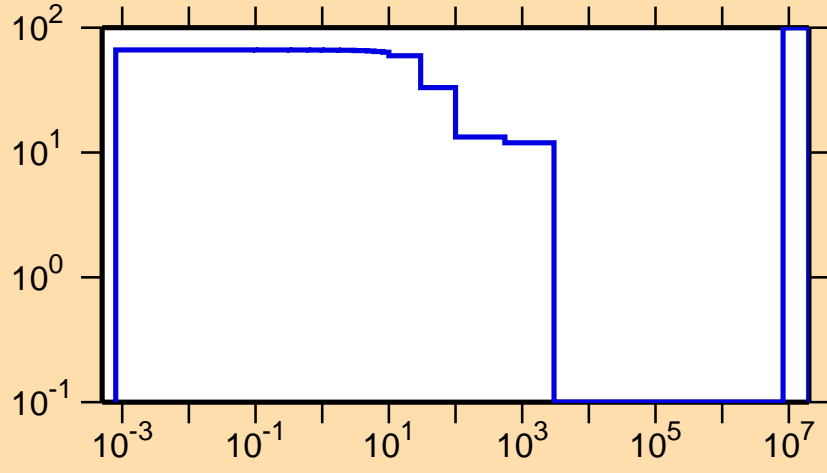
\Delta\sigma/\sigma vs. E for ^{220}\text{Rn}(n,f)
