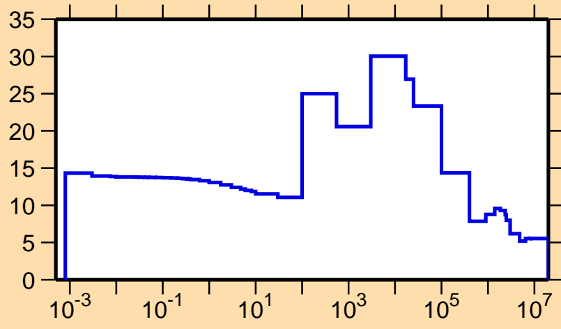
\sigma vs. E for ^{220}\text{Rn}(n,\text{el.})
