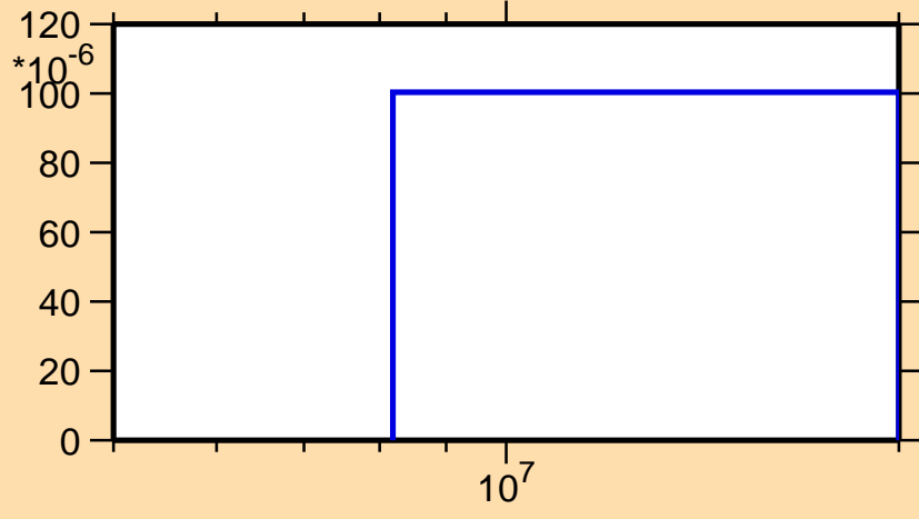
\sigma vs. E for ^{220}\text{Rn}(n,d)
