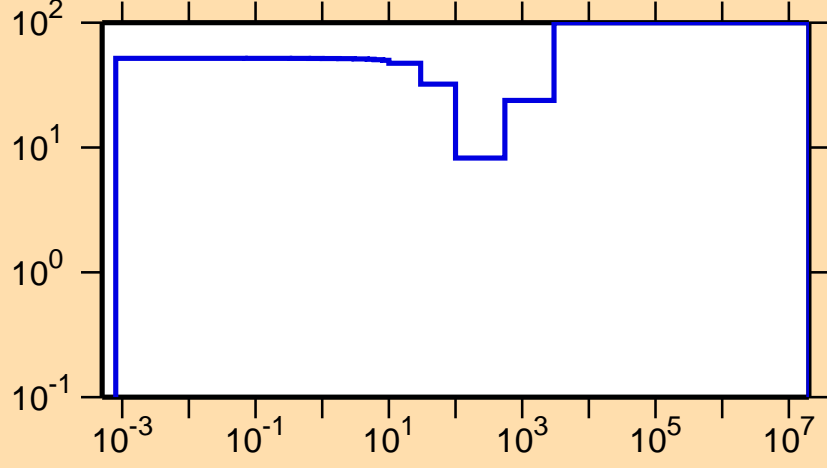
\Delta\sigma/\sigma vs. E for ^{220}\text{Rn}(n,\gamma)
