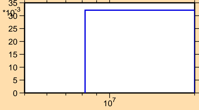
\sigma vs. E for ^{220}\text{Rn}(n,3n)
