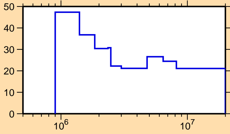
\Delta\sigma/\sigma vs. E for ^{220}\text{Rn}(n,\text{nonel.})
