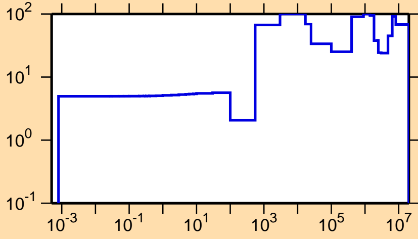
\Delta\sigma/\sigma vs. E for ^{220}\text{Rn}(n,el.)
