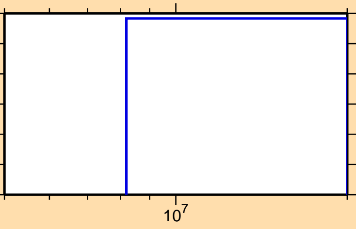
\sigma vs. E for ^{220}\text{Rn}(\text{mt117})
