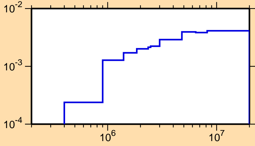
\sigma vs. E for ^{220}\text{Rn}(n,n_3)
