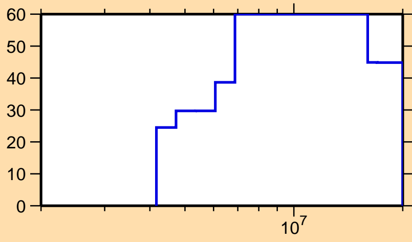
\Delta\sigma/\sigma vs. E for ^{221}\text{Rn}(n,\text{el.})
