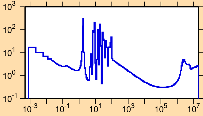
\sigma vs. E for ^{221}\text{Rn}(n,\text{nonel.})
