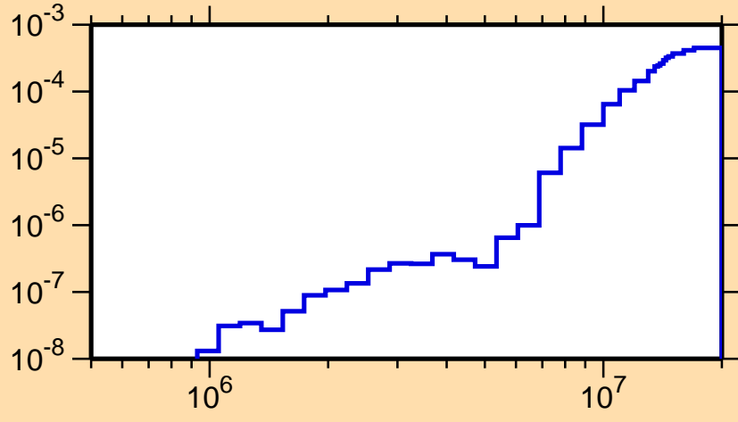
\sigma vs. E for ^{221}\text{Rn}(n,n\alpha)
