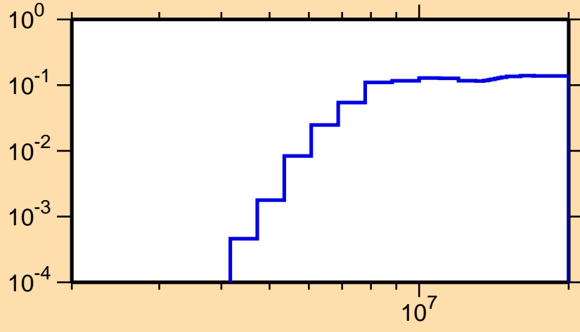
\sigma vs. E for ^{221}\text{Rn}(n,2n)
