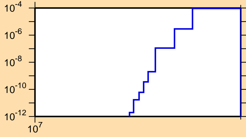
\sigma vs. E for ^{221}\text{Rn}(n,2np)
