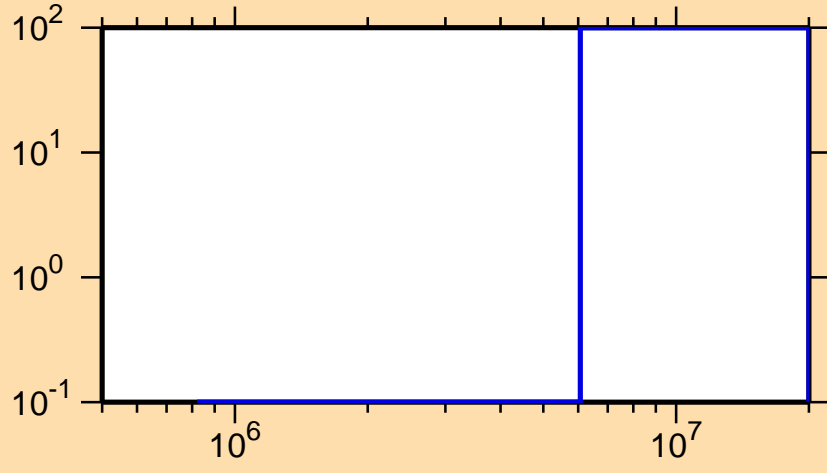
\Delta\sigma/\sigma vs. E for ^{221}\text{Rn}(n,f)
