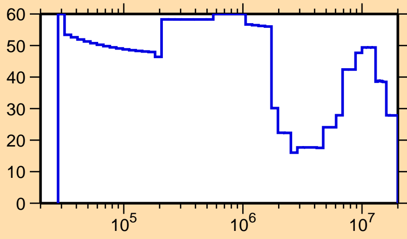
\Delta\sigma/\sigma vs. E for ^{221}\text{Rn}(n,\text{tot.})
