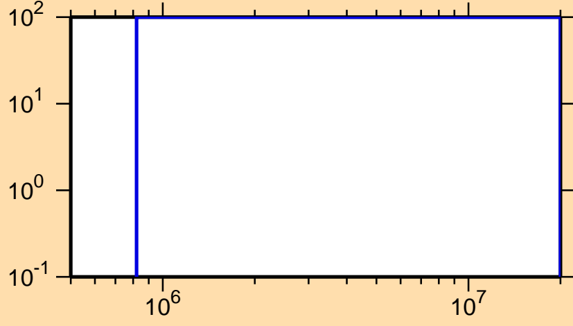
\Delta\sigma/\sigma vs. E for ^{221}\text{Rn}(n,n\text{cont.})
