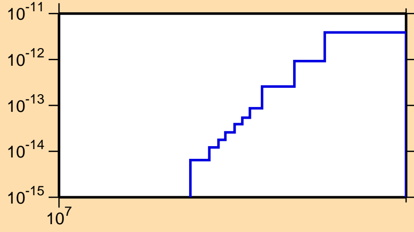
\sigma vs. E for ^{221}\text{Rn}(n,p\alpha)
