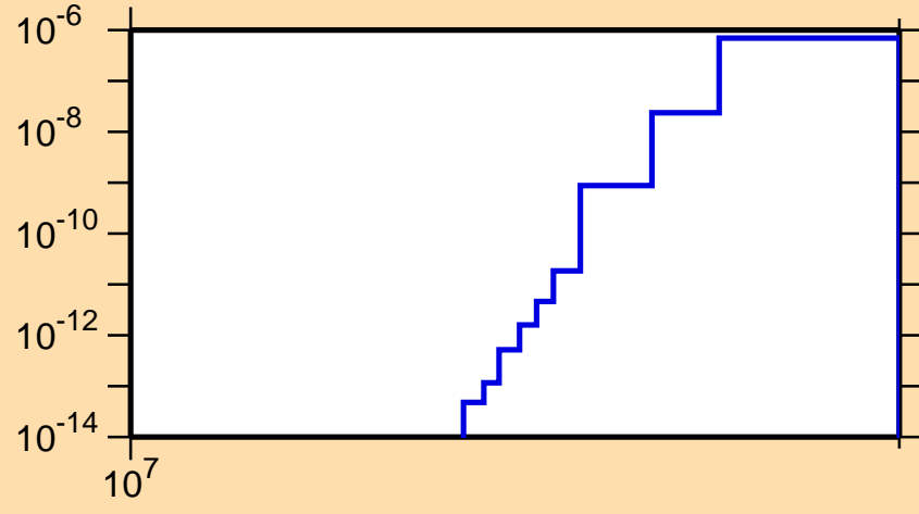
\sigma vs. E for ^{221}\text{Rn}(n,nt)
