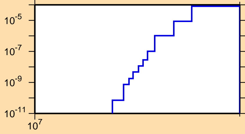
\sigma vs. E for ^{221}\text{Rn}(n,nd)
