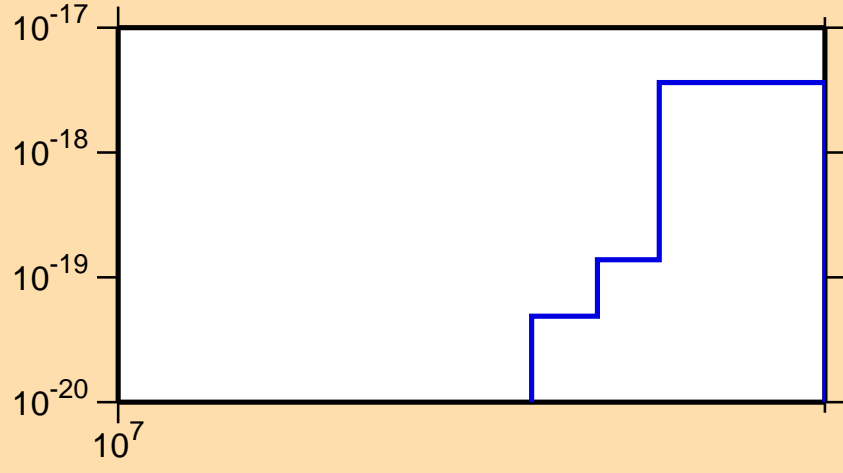
\sigma vs. E for ^{221}\text{Rn}(\text{mt } 11)
