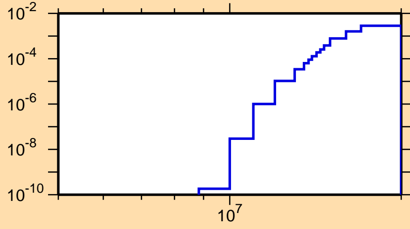
\sigma vs. E for ^{221}\text{Rn}(n,d)
