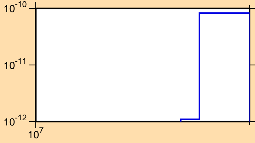
\sigma vs. E for ^{221}\text{Rn}(n,\text{He}3)
