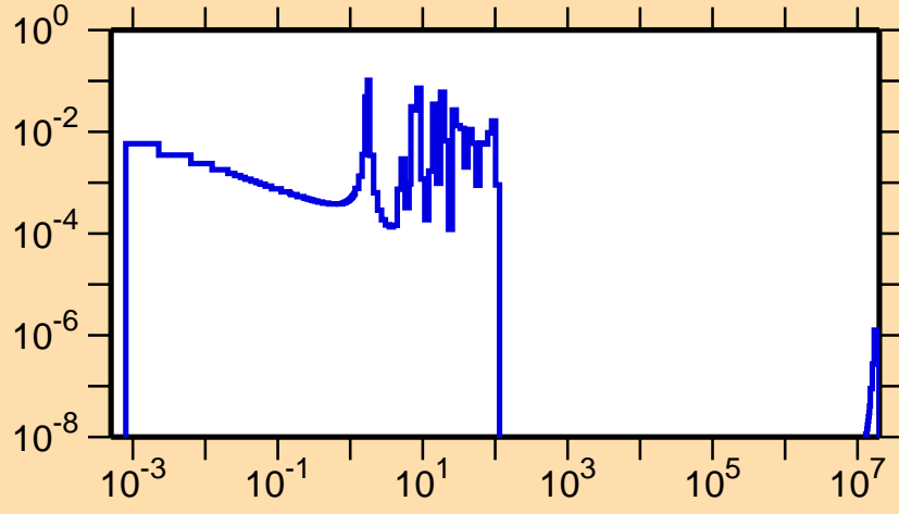
\sigma vs. E for ^{221}\text{Rn}(n,f)
