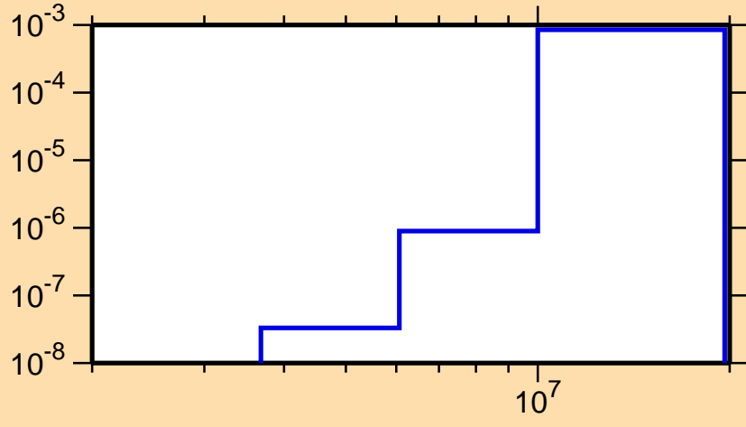
\sigma vs. E for ^{221}\text{Rn}(n,p)
