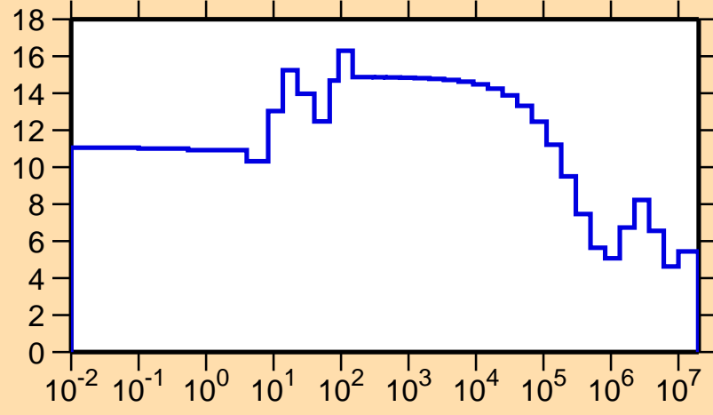
\sigma vs. E for ^{221}\text{Rn}(n,\text{el.})
