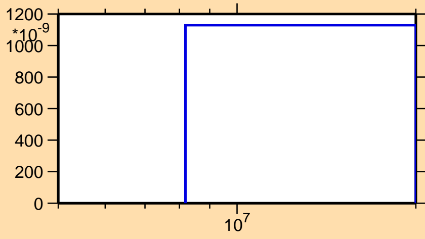
\sigma vs. E for ^{221}\text{Rn}(n,\text{nd})
