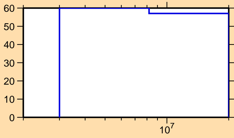
\Delta\sigma/\sigma vs. E for ^{221}\text{Rn}(n,2n)
