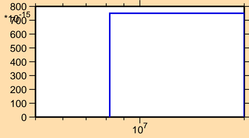
\sigma vs. E for ^{221}\text{Rn}(n,\text{He}3)
