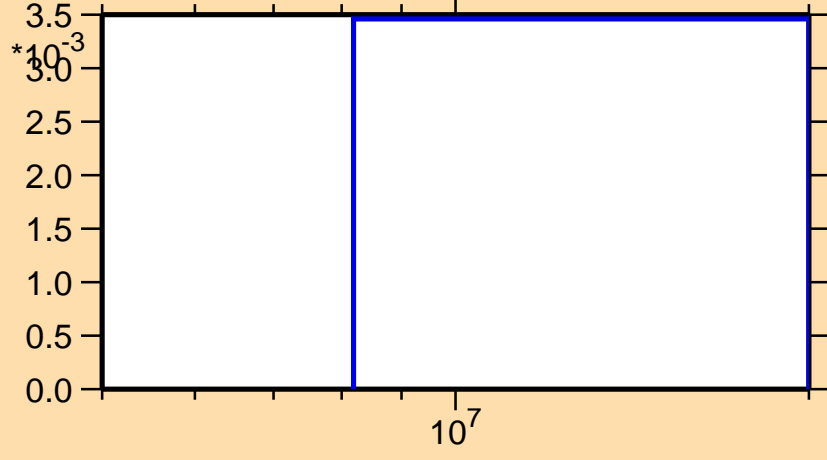
\sigma vs. E for ^{221}\text{Rn}(n,3n)
