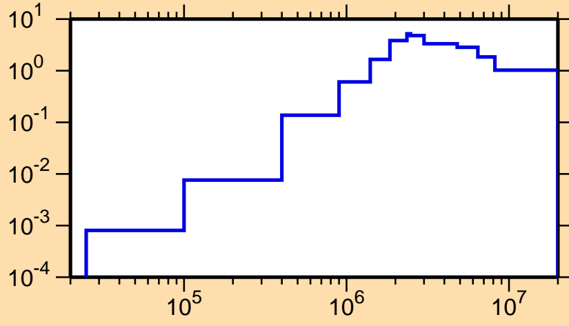
\sigma vs. E for ^{221}\text{Rn}(n,\text{inel.})
