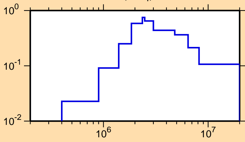
\sigma vs. E for ^{221}\text{Rn}(n,n_4)
