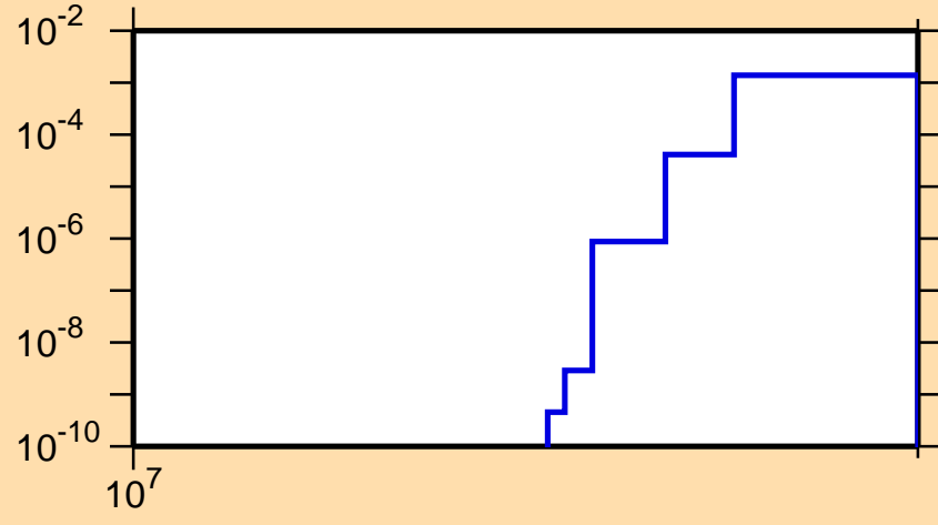
\sigma vs. E for ^{222}\text{Rn}(n,nd)
