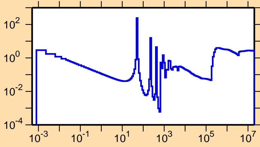
\sigma vs. E for ^{222}\text{Rn}(n,\text{nonel.})
