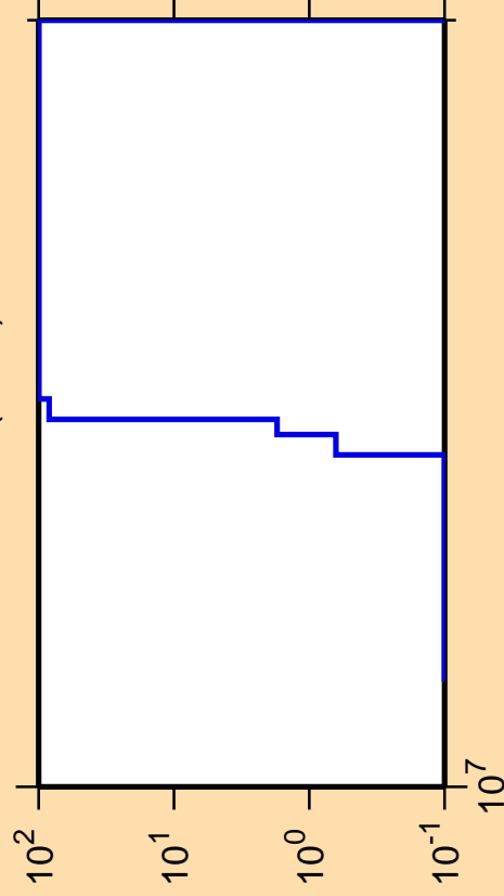
\Delta\sigma/\sigma vs. E for ^{222}\text{Rn}(n,nd)
