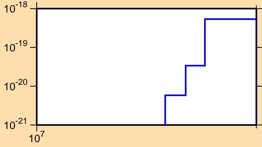
\sigma vs. E for ^{222}\text{Rn} (mt 11)
