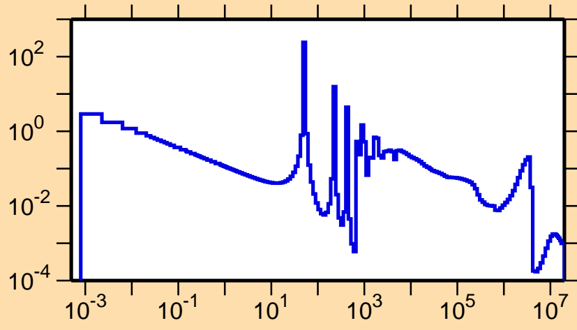
\sigma vs. E for ^{222}\text{Rn}(n,\gamma)
