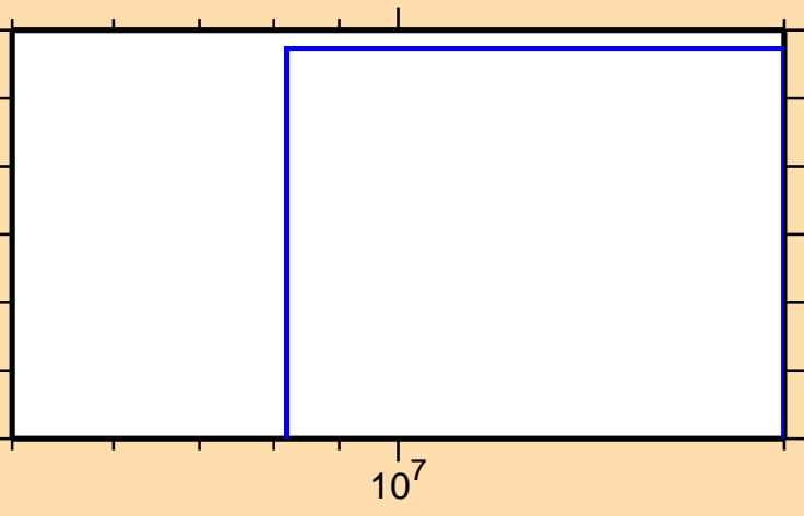
\sigma vs. E for ^{222}\text{Rn}(n,2np)
