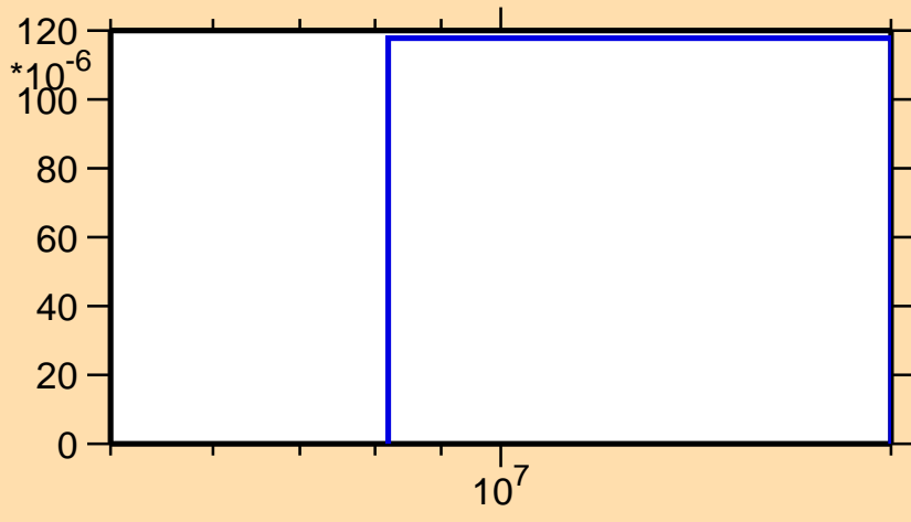
\sigma vs. E for ^{222}\text{Rn}(n,d)
