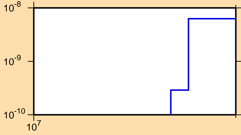
\sigma vs. E for ^{223}\text{Rn}(n,\text{He}3)
