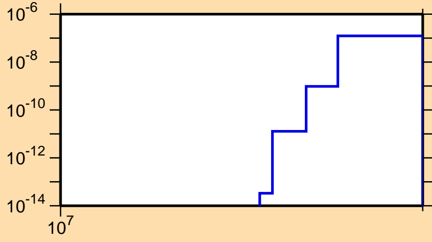
\sigma vs. E for ^{223}\text{Rn}(n,2np)
