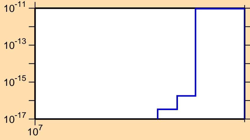
\sigma vs. E for ^{223}\text{Rn} (mt 11)
