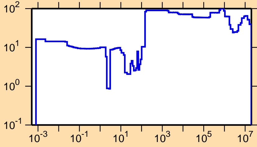
\Delta\sigma/\sigma vs. E for ^{223}\text{Rn}(n,tot.)
