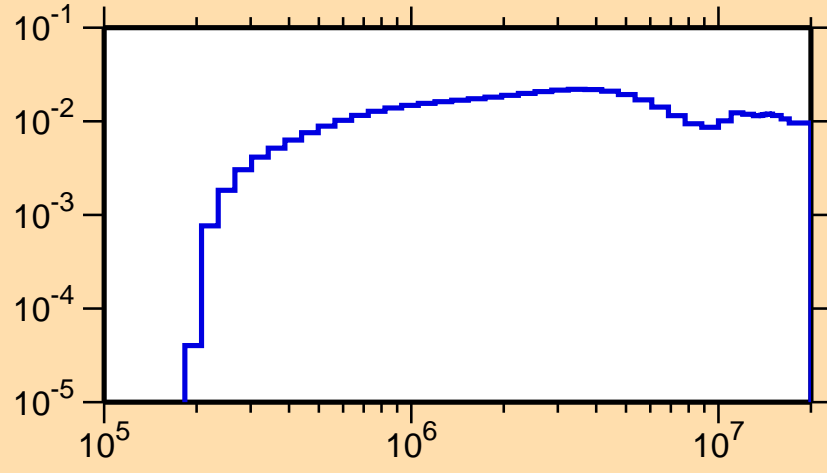
\sigma vs. E for ^{223}\text{Rn}(n,n_1)
