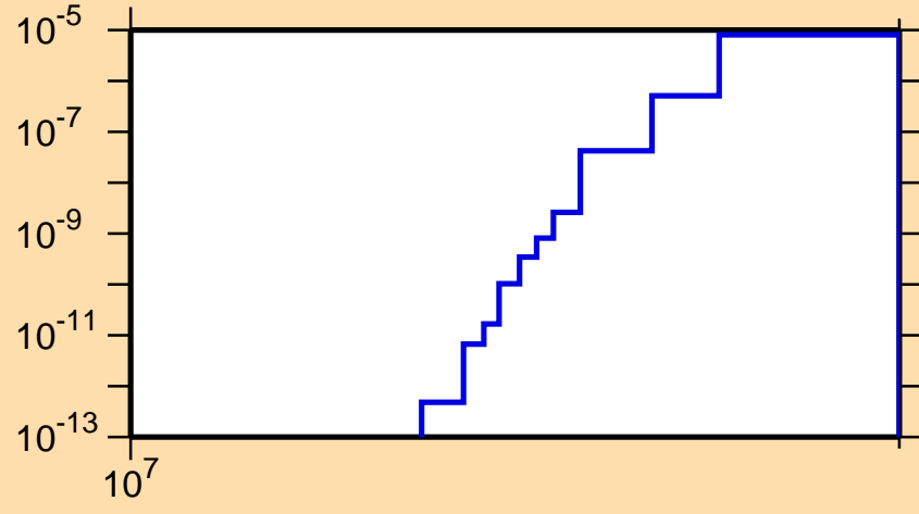
\sigma vs. E for ^{223}\text{Rn}(n,\text{nd})
