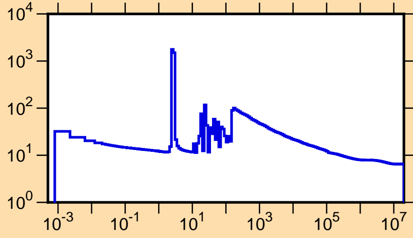
\sigma vs. E for ^{223}\text{Rn}(n,\text{tot.})
