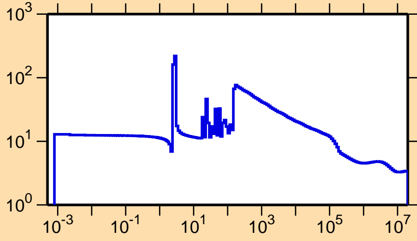
\sigma vs. E for ^{223}\text{Rn}(n,\text{el.})
