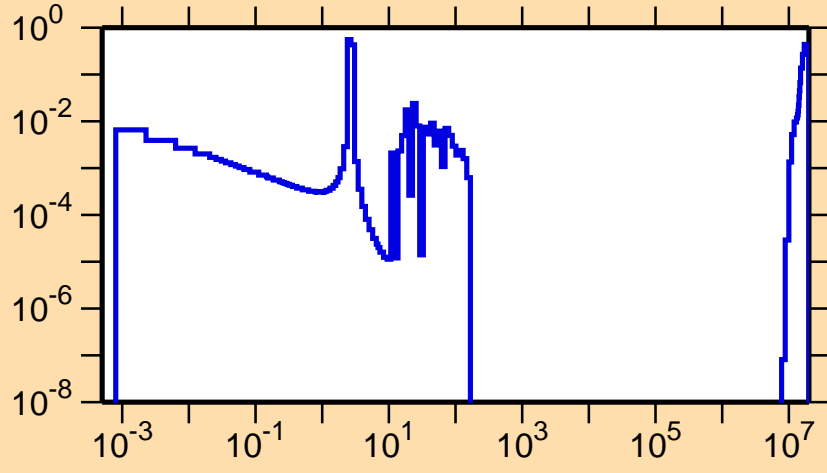
\sigma vs. E for ^{223}\text{Rn}(n,f)
