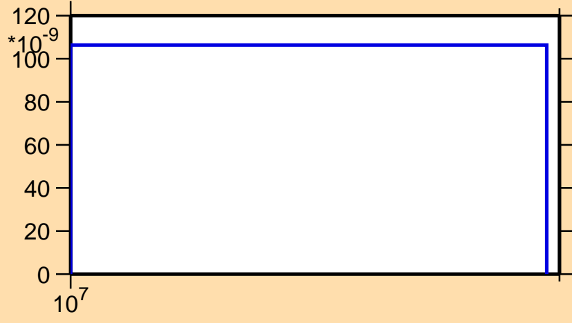
\sigma vs. E for ^{223}\text{Rn}(n,\text{nd})
