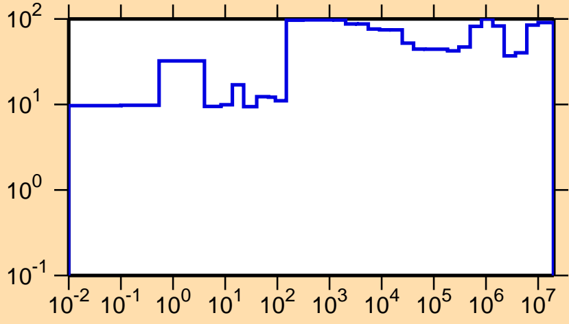
\Delta\sigma/\sigma vs. E for ^{223}\text{Rn}(n,\text{el.})
