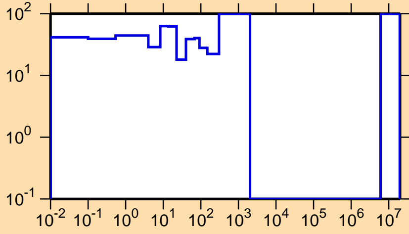
\Delta\sigma/\sigma vs. E for ^{223}\text{Rn}(n,f)
