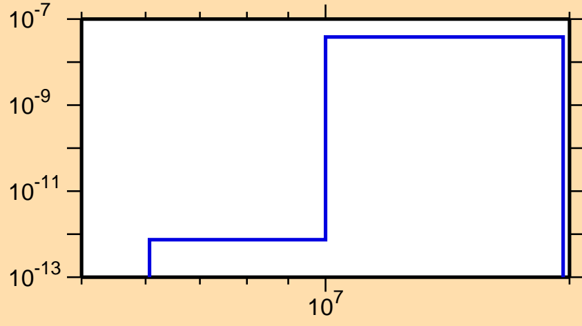
\sigma vs. E for ^{223}\text{Rn}(n,2n\alpha)
