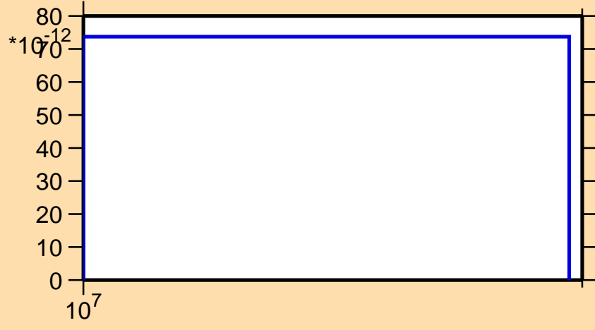
\sigma vs. E for ^{223}\text{Rn}(n,\text{He}3)
