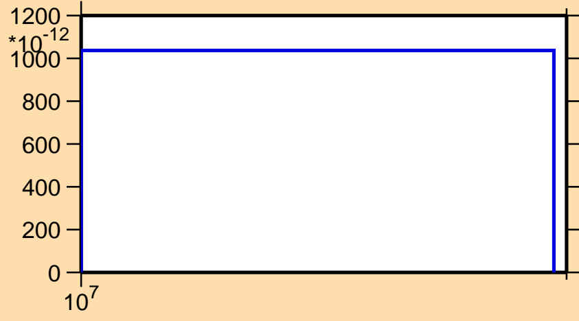
\sigma vs. E for ^{223}\text{Rn}(n,2np)
