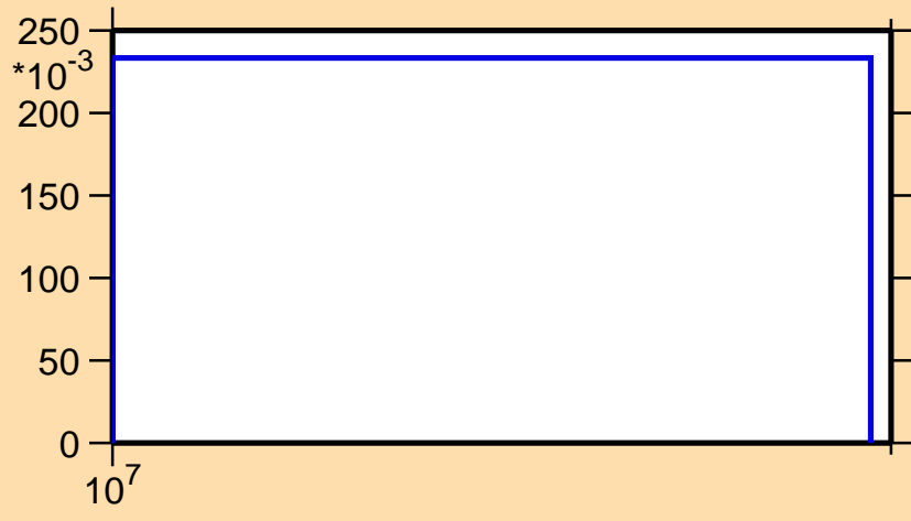
\sigma vs. E for ^{223}\text{Rn}(n,3n)
