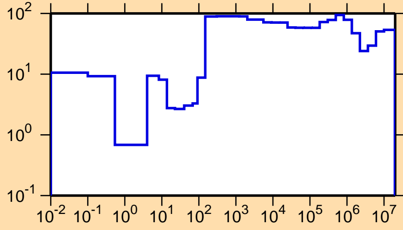
\Delta\sigma/\sigma vs. E for ^{223}\text{Rn}(n,\text{tot.})
