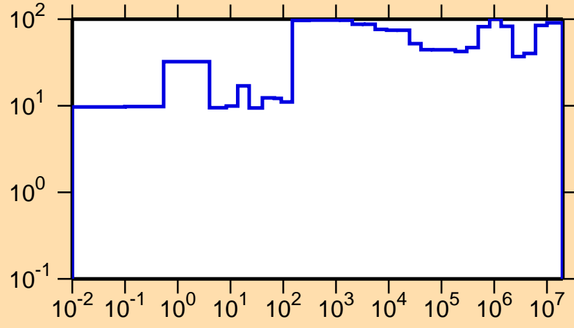
\Delta\sigma/\sigma vs. E for ^{223}\text{Rn}(n,el.)
