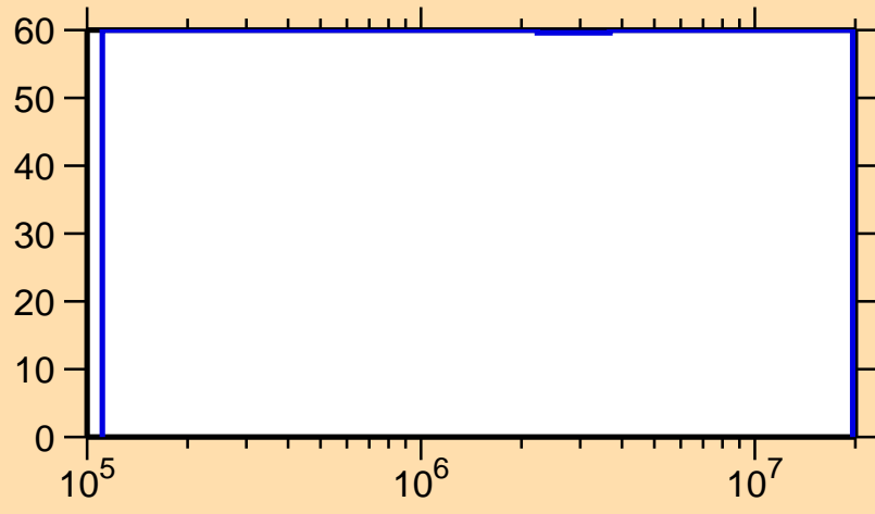
\Delta\sigma/\sigma vs. E for ^{223}\text{Rn}(n,n\text{cont.})
