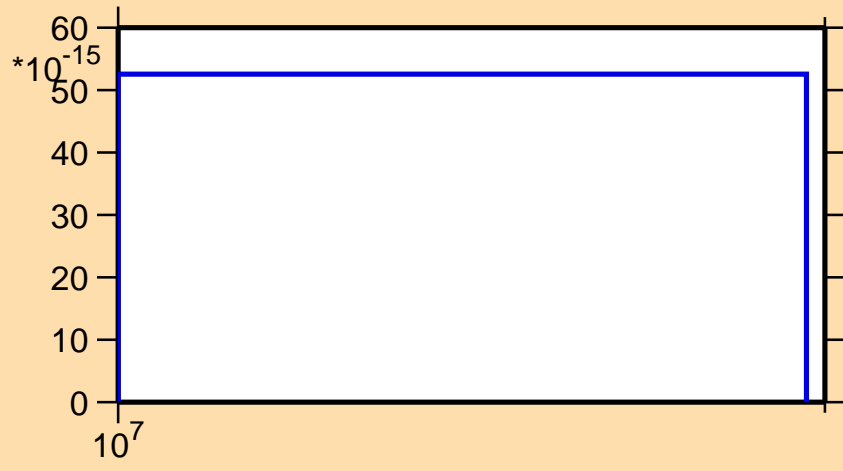
\sigma vs. E for ^{223}\text{Rn} (mt 11)
