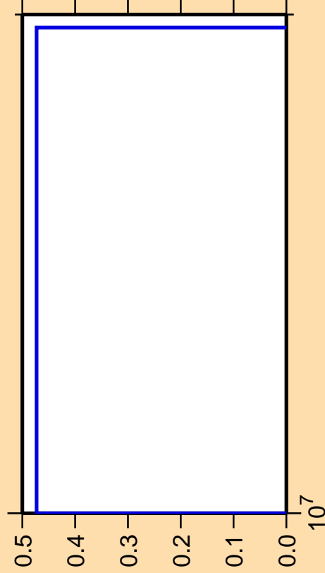
\Delta\sigma/\sigma vs. E for ^{223}\text{Rn} (mt 11)
