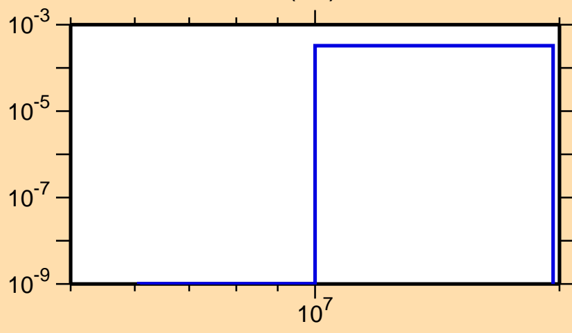
\sigma vs. E for ^{223}\text{Rn}(n,t)
