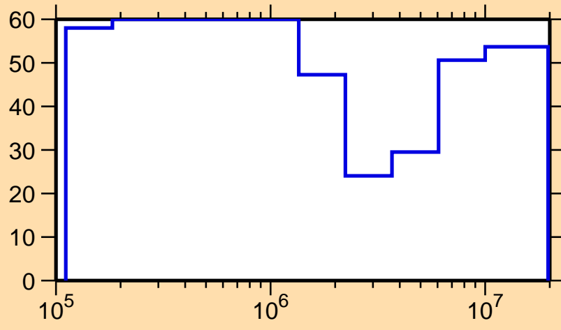
\Delta\sigma/\sigma vs. E for ^{223}\text{Rn}(n,\text{tot.})
