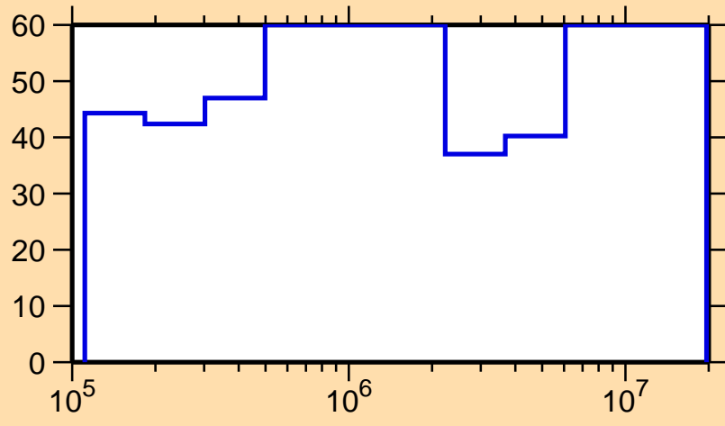
\Delta\sigma/\sigma vs. E for ^{223}\text{Rn}(n,\text{el.})
