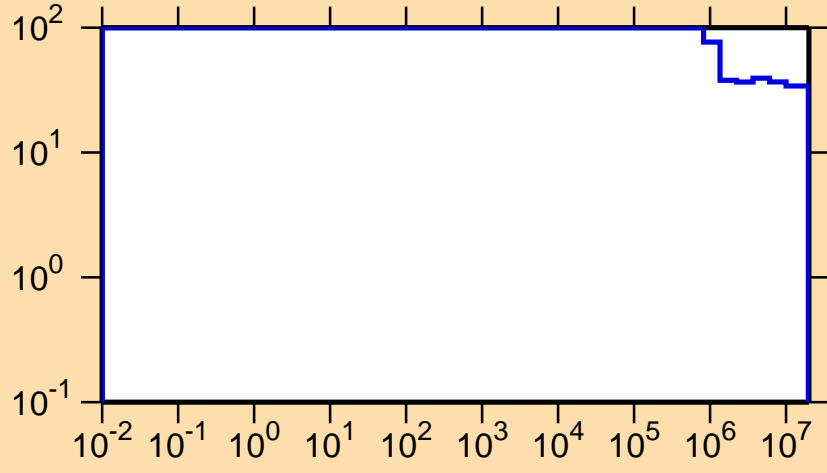
\Delta\sigma/\sigma vs. E for ^{223}\text{Rn}(n,\text{nonel.})
