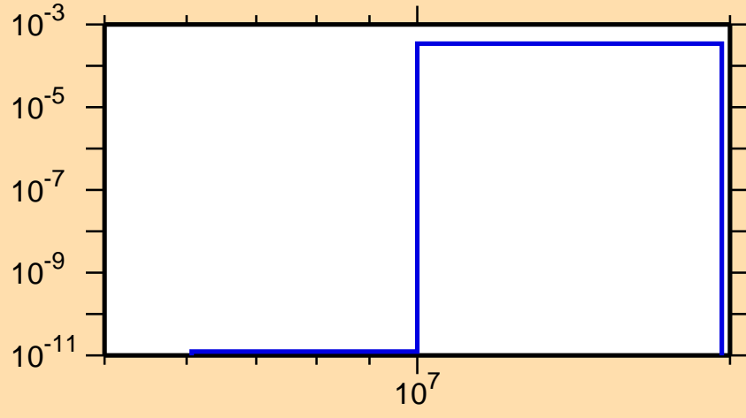
\sigma vs. E for ^{223}\text{Rn}(n,d)
