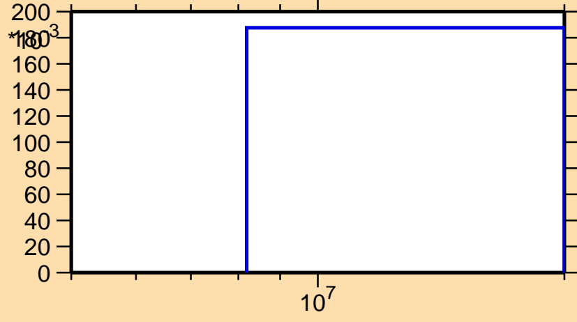
\sigma vs. E for ^{223}\text{Rn}(n,3n)
