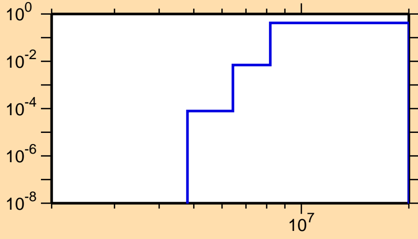
\sigma vs. E for ^{223}\text{Rn}(n,2n)
