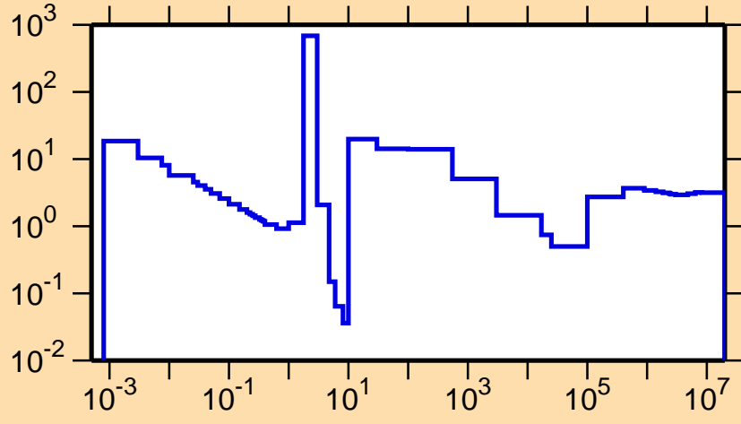
\sigma vs. E for ^{223}\text{Rn}(n,\text{nonel.})
