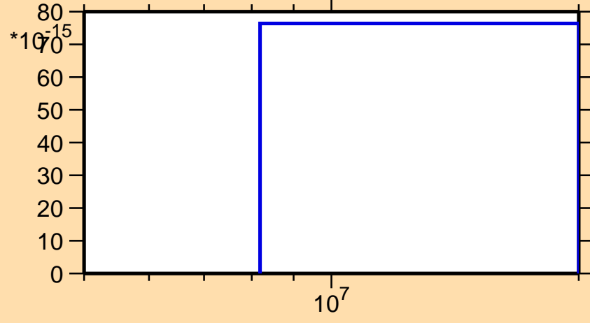
\sigma vs. E for ^{223}\text{Rn}(\text{mt } 11)
