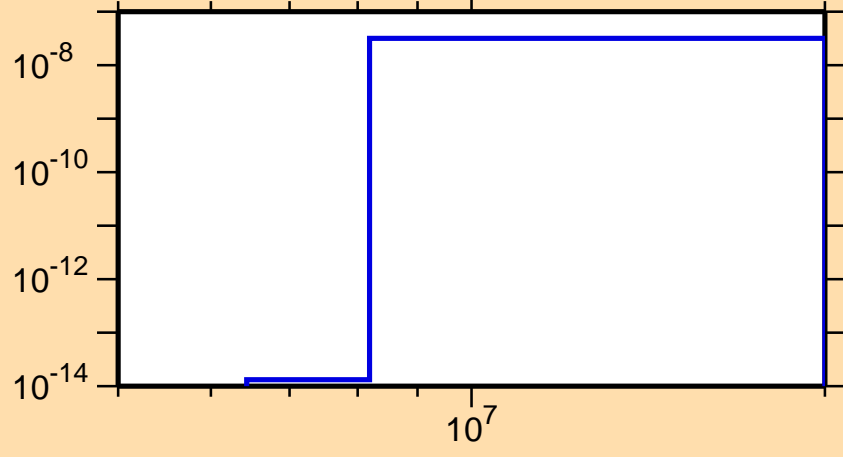
\sigma vs. E for ^{223}\text{Rn}(n,2n\alpha)
