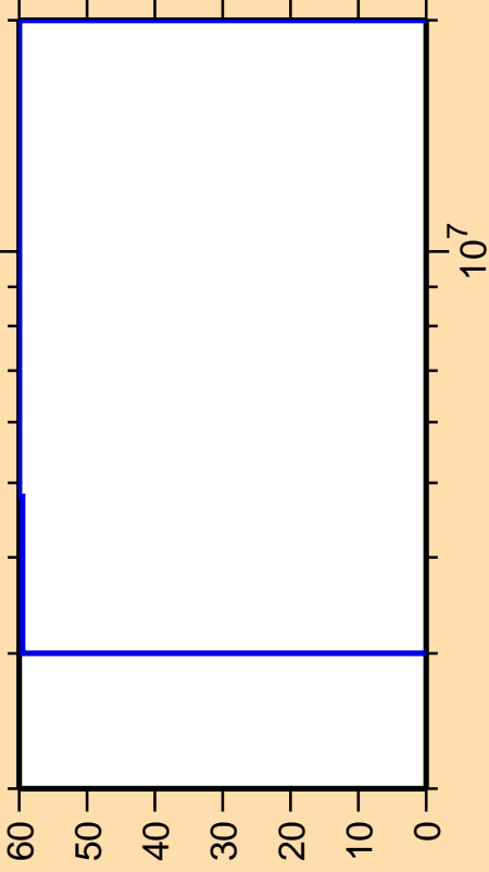
\Delta\sigma/\sigma vs. E for ^{223}\text{Rn}(n,n\text{cont.})
