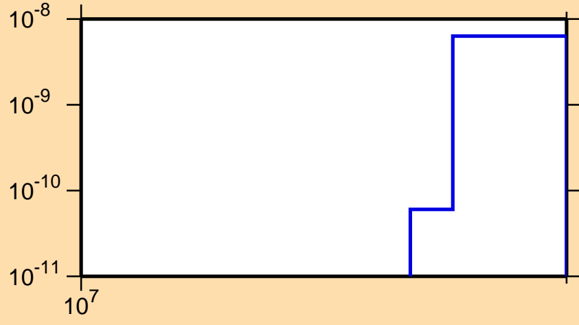
\sigma vs. E for ^{224}\text{Rn}(n,nd)
