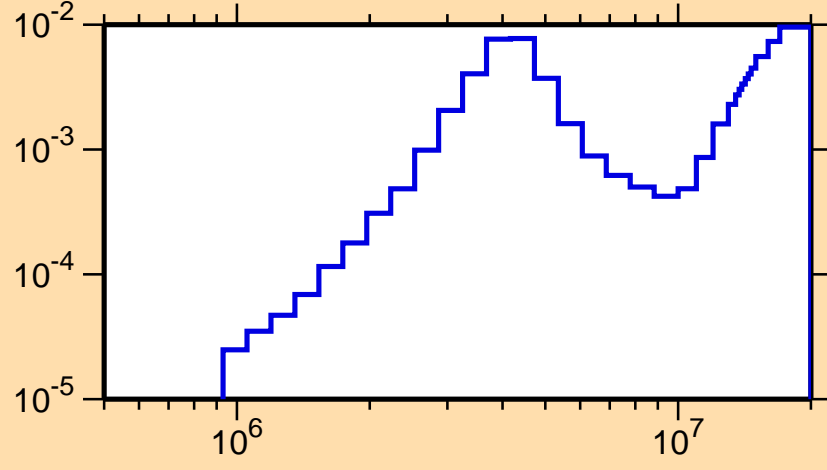
\sigma vs. E for ^{224}\text{Rn}(n,\alpha)
