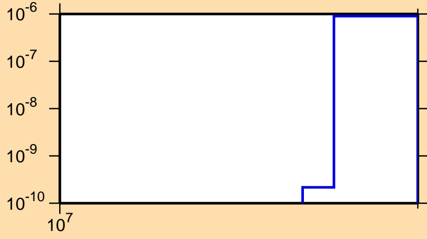
\sigma vs. E for ^{224}\text{Rn}(n,2np)
