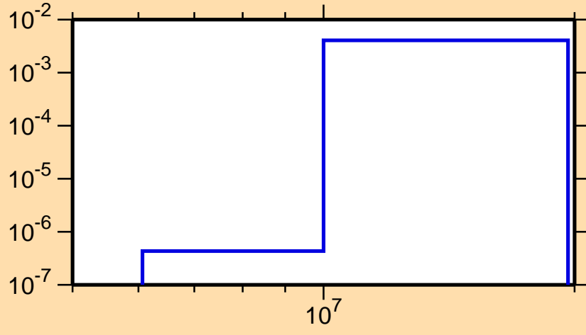
\sigma vs. E for ^{224}\text{Rn}(n,p)
