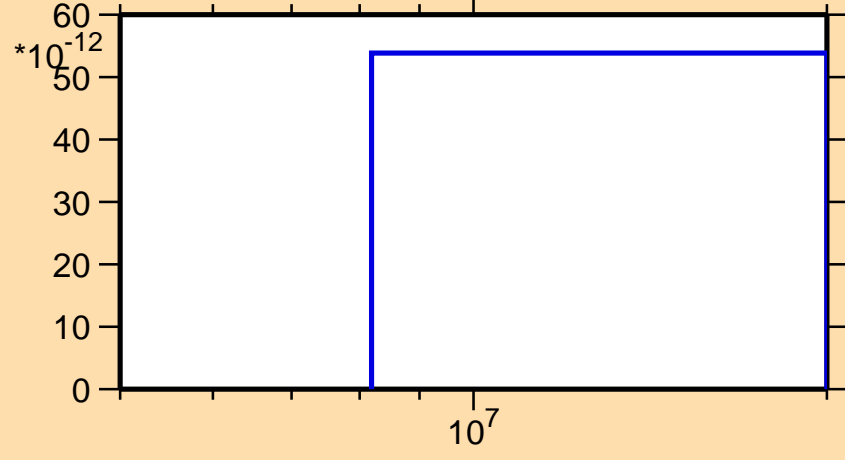
\sigma vs. E for ^{224}\text{Rn}(n,nd)
