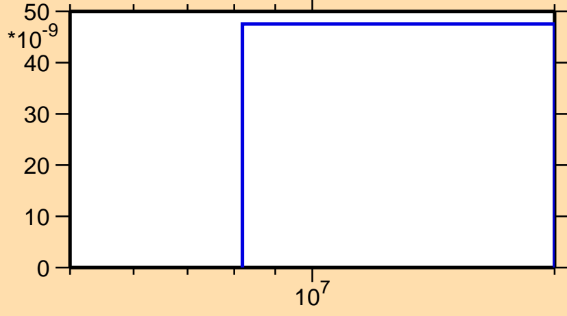
\sigma vs. E for ^{224}\text{Rn}(n,np)
