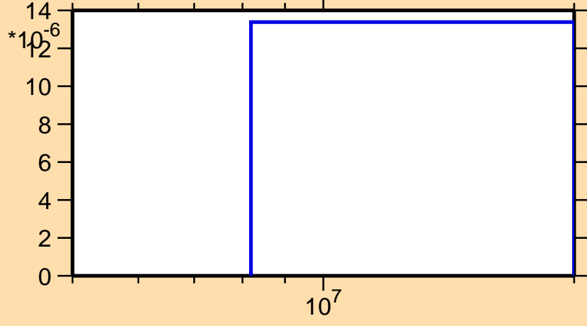
\sigma vs. E for ^{224}\text{Rn}(n,d)
