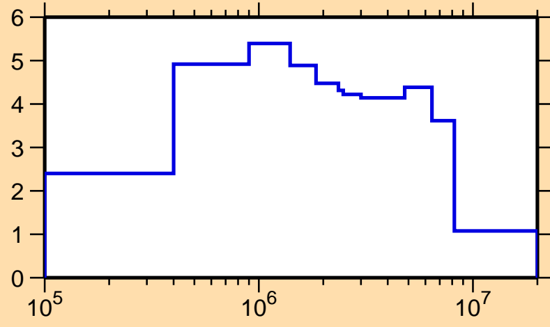
\sigma vs. E for ^{224}\text{Rn}(n,\text{inel.})
