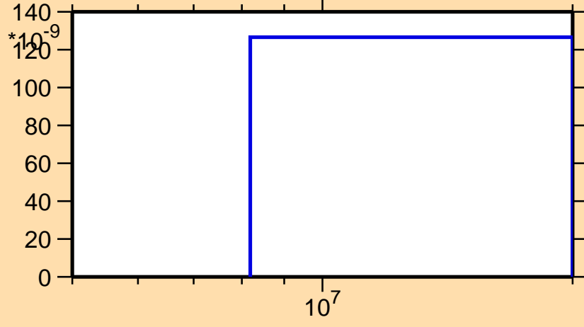
\sigma vs. E for ^{224}\text{Rn}(n,3n\alpha)
