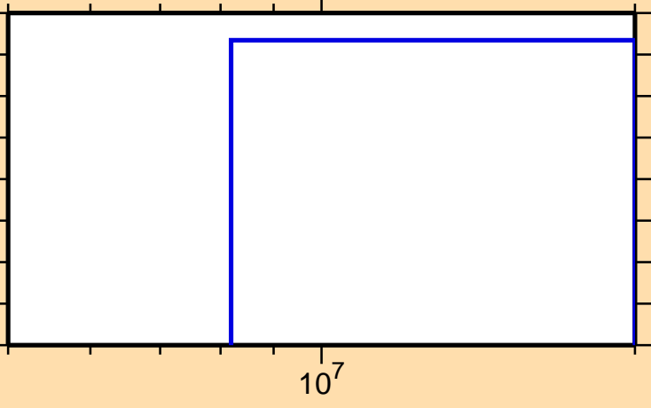
\sigma vs. E for ^{224}\text{Rn}(n,2np)
