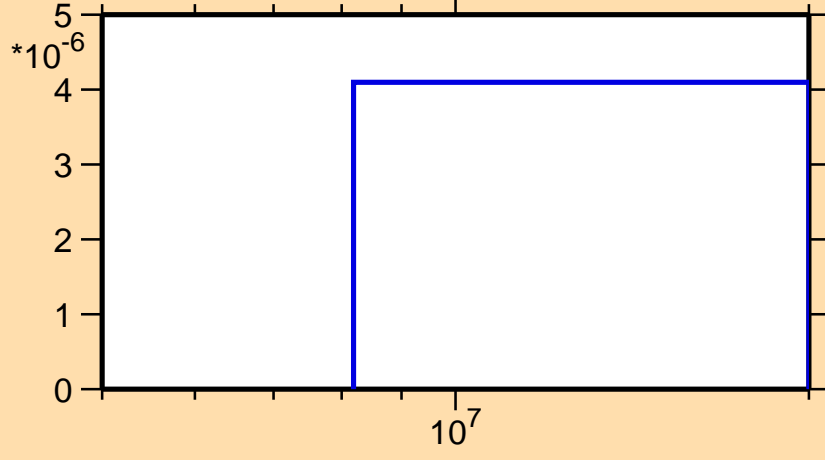
\sigma vs. E for ^{224}\text{Rn}(n,2n\alpha)
