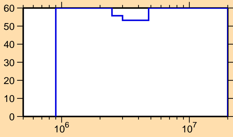
\Delta\sigma/\sigma vs. E for ^{224}\text{Rn}(n,n\text{cont.})
