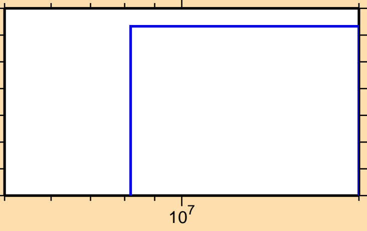
\sigma vs. E for ^{224}\text{Rn}(n,3n\alpha)
