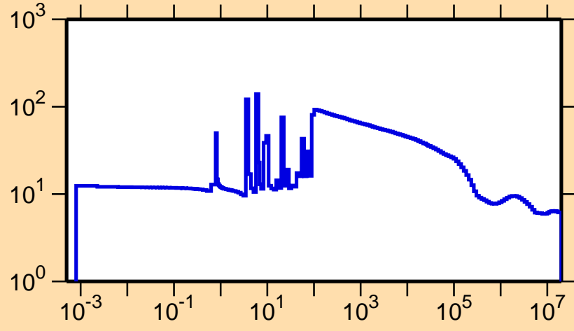
\sigma vs. E for ^{225}\text{Rn}(n,\text{el.})
