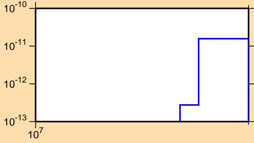
\sigma vs. E for ^{225}\text{Rn}(n,\text{He}3)
