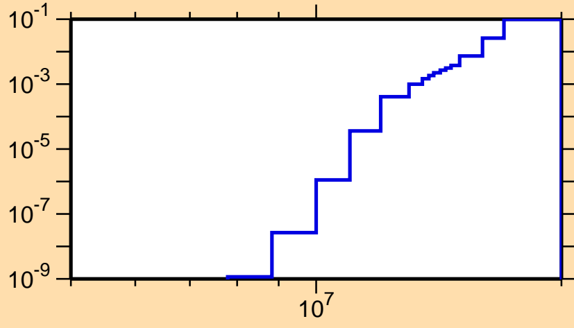
\sigma vs. E for ^{225}\text{Rn}(n,2n\alpha)
