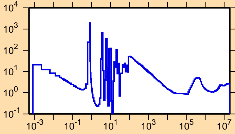
\sigma vs. E for ^{225}\text{Rn}(n,\text{nonel.})
