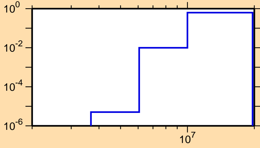
\sigma vs. E for ^{225}\text{Rn}(n,p)
