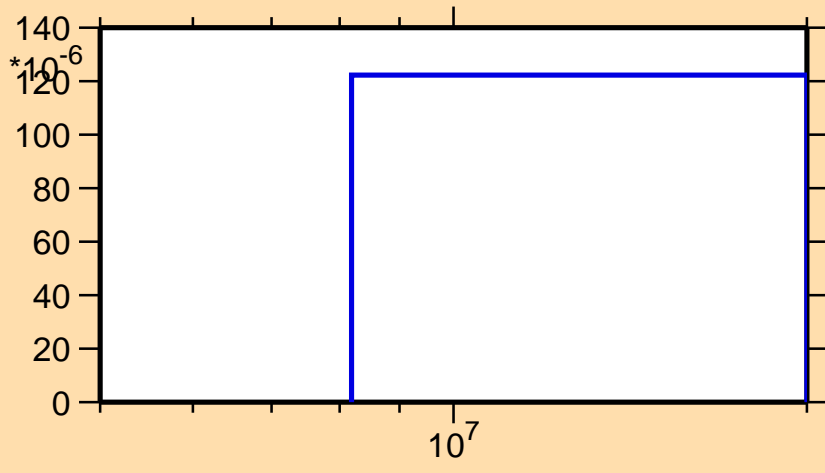
\sigma vs. E for ^{225}\text{Rn}(n,t)
