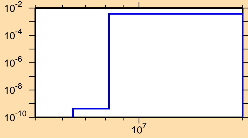
\sigma vs. E for ^{225}\text{Rn}(n,2n\alpha)
