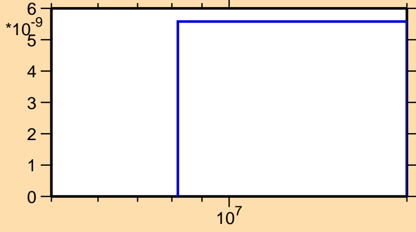
\sigma vs. E for ^{225}\text{Rn}(n,2np)
