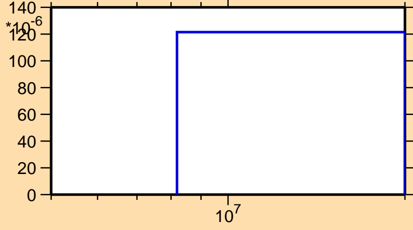
\sigma vs. E for ^{225}\text{Rn}(n,d)
