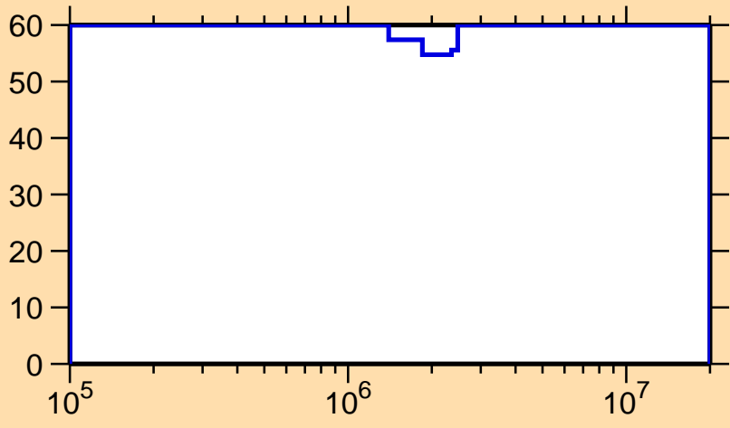
\Delta\sigma/\sigma vs. E for ^{225}\text{Rn}(n,\text{inel.})
