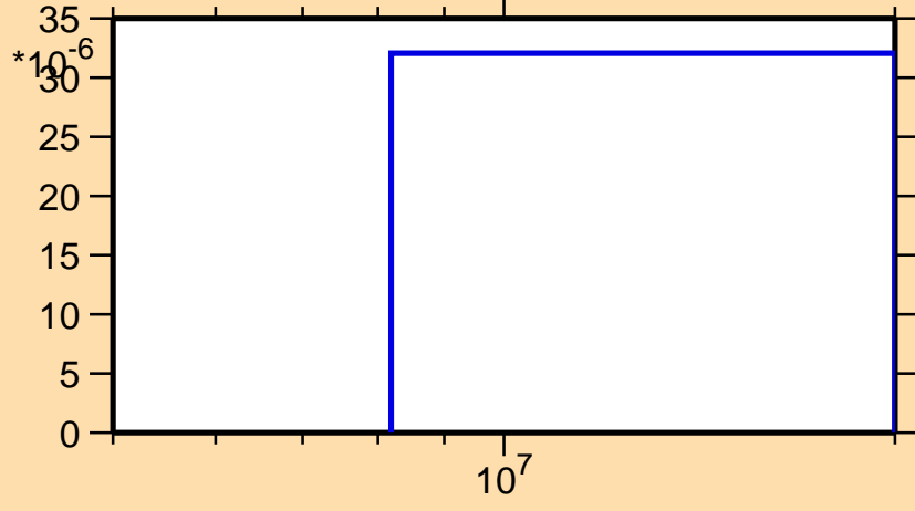
\sigma vs. E for ^{225}\text{Rn}(n,3n)
