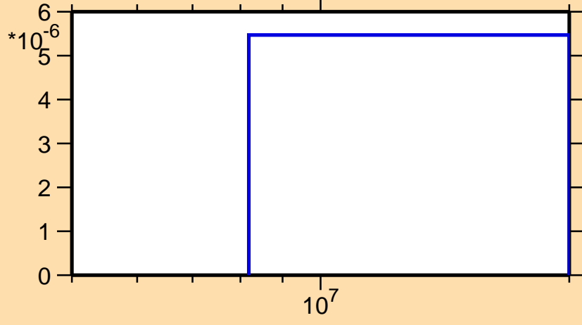
\sigma vs. E for ^{225}\text{Rn}(n,np)
