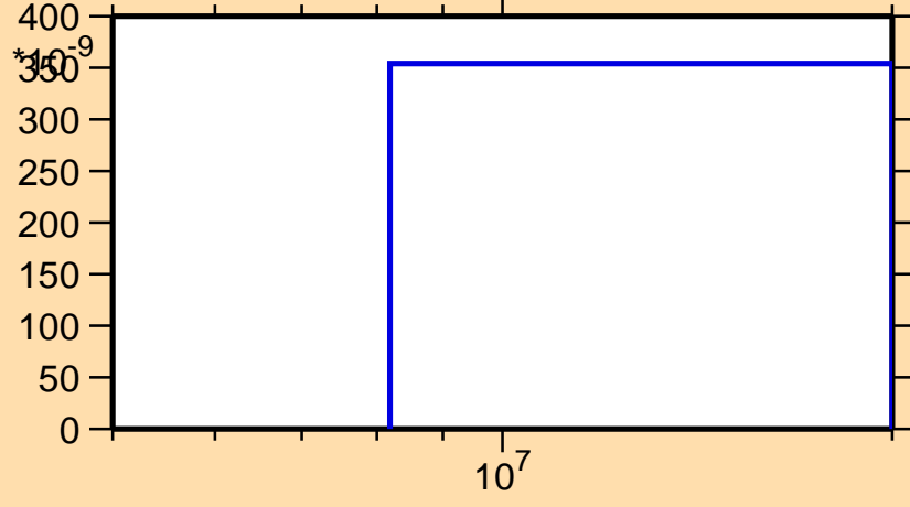
\sigma vs. E for ^{225}\text{Rn}(n,\text{nd})
