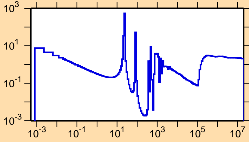
\sigma vs. E for ^{226}\text{Rn}(n,\text{nonel.})
