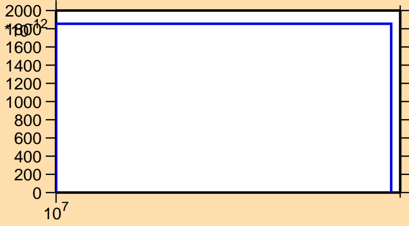
\sigma vs. E for ^{226}\text{Rn}(n,nd)
