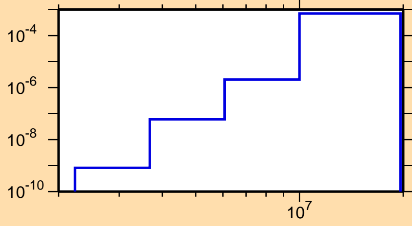
\sigma vs. E for ^{226}\text{Rn}(n,\alpha)
