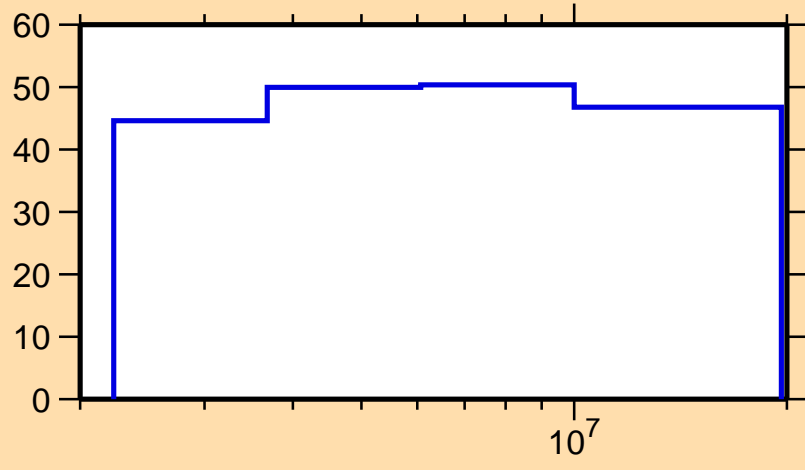
\Delta\sigma/\sigma vs. E for ^{226}\text{Rn}(n,\text{nonel.})
