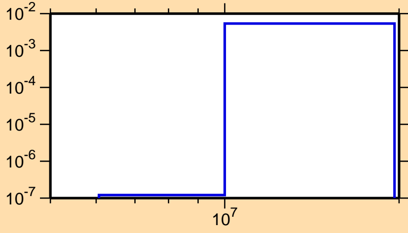
\sigma vs. E for ^{226}\text{Rn}(n,p)
