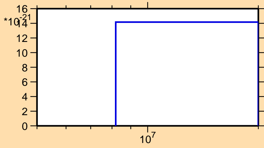
\sigma vs. E for ^{226}\text{Rn} (mt 42)
