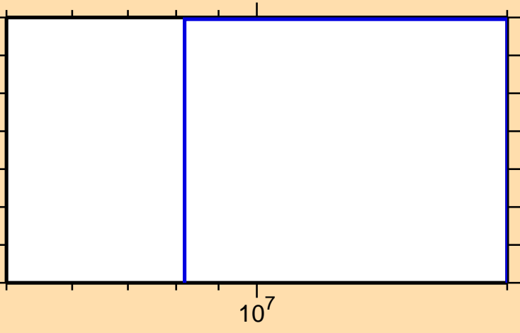
\sigma vs. E for ^{226}\text{Rn}(n,t)
