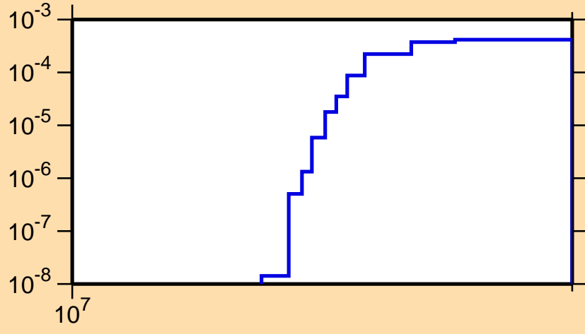
\sigma vs. E for ^{227}\text{Rn}(n,nd)
