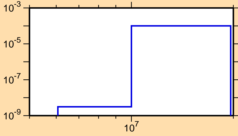
\sigma vs. E for ^{227}\text{Rn}(n,n\alpha)
