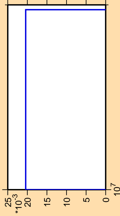
\Delta\sigma/\sigma vs. E for ^{227}\text{Rn}(n,3n\alpha)
