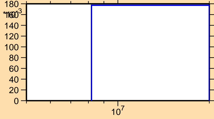
\sigma vs. E for ^{227}\text{Rn}(n,3n)
