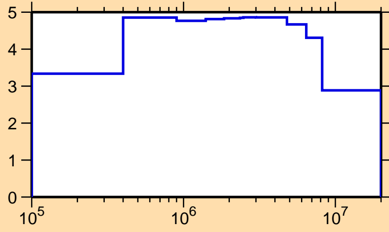
\sigma vs. E for ^{227}\text{Rn}(n,\text{inel.})
