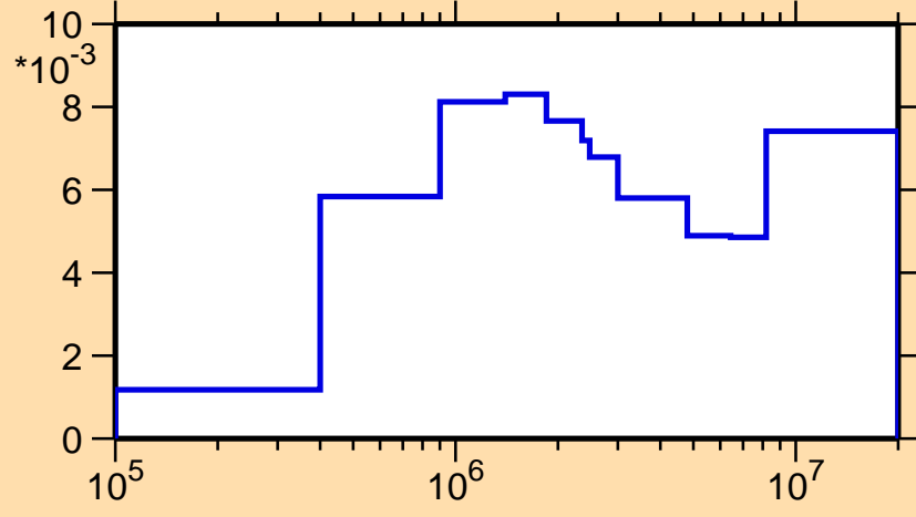
\sigma vs. E for ^{227}\text{Rn}(n,n_1)
