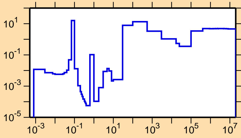
\sigma vs. E for ^{227}\text{Rn}(n,\text{nonel.})
