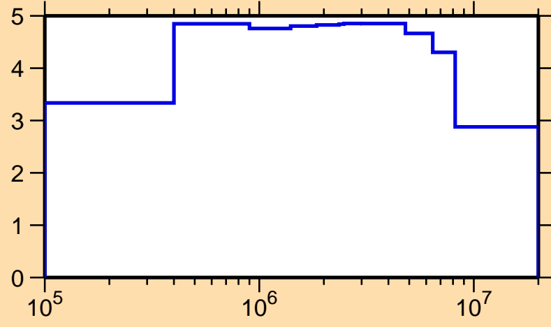
\sigma vs. E for ^{227}\text{Rn}(n,n\text{cont.})
