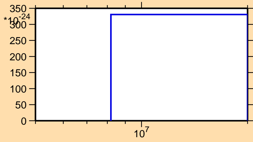
\sigma vs. E for ^{227}\text{Rn} (mt 42)
