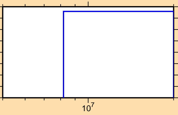
\sigma vs. E for ^{227}\text{Rn}(n,d)
