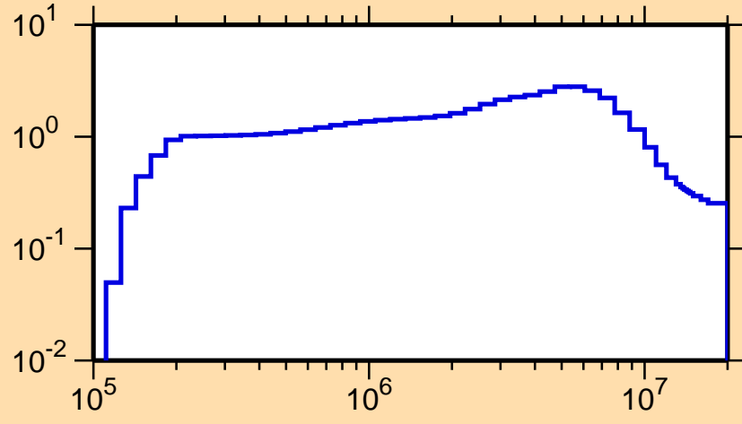
\sigma vs. E for ^{228}\text{Rn}(n,\text{inel.})
