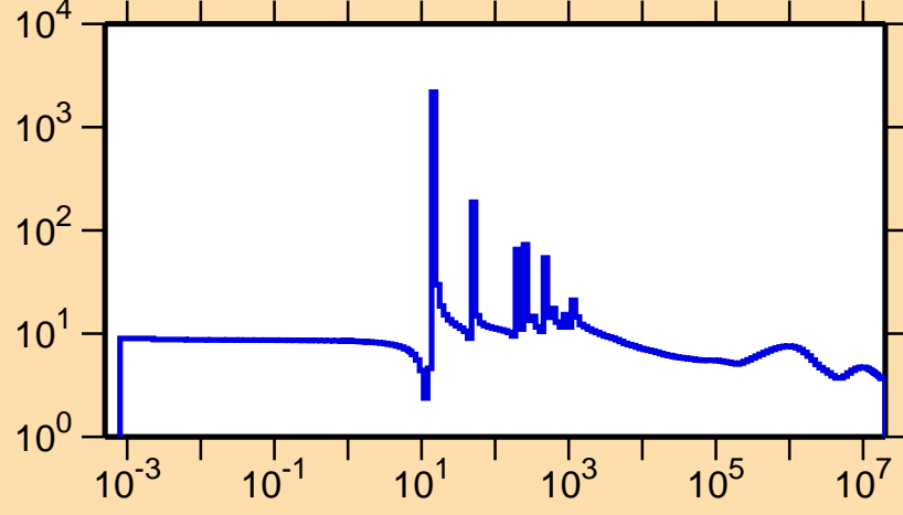
\sigma vs. E for ^{228}\text{Rn}(n,\text{el.})
