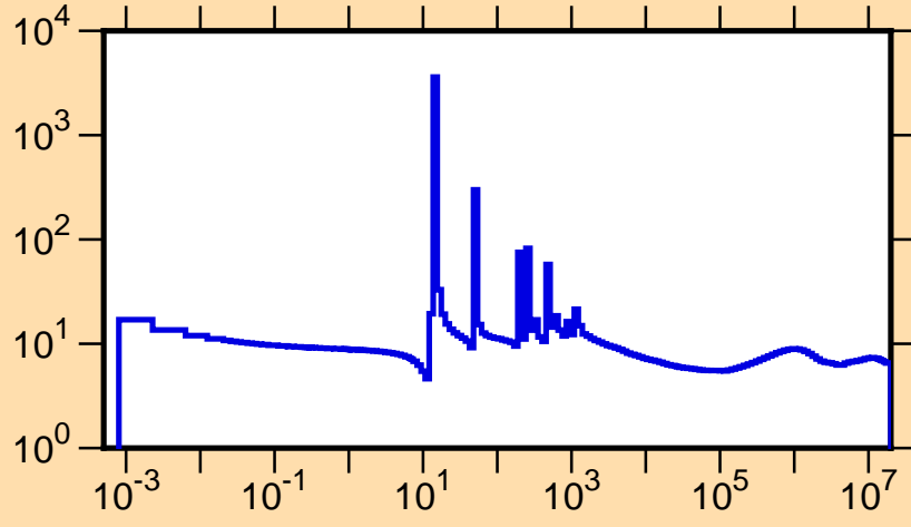
\sigma vs. E for ^{228}\text{Rn}(n,\text{tot.})
