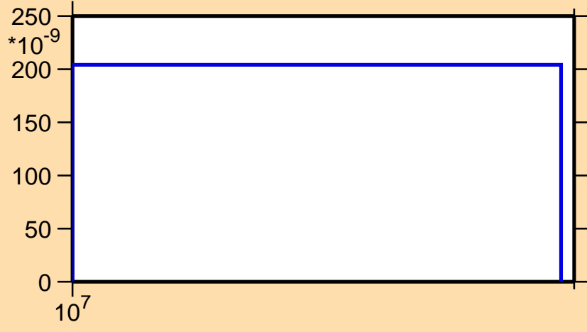
\sigma vs. E for ^{228}\text{Rn}(n,2n\alpha)
