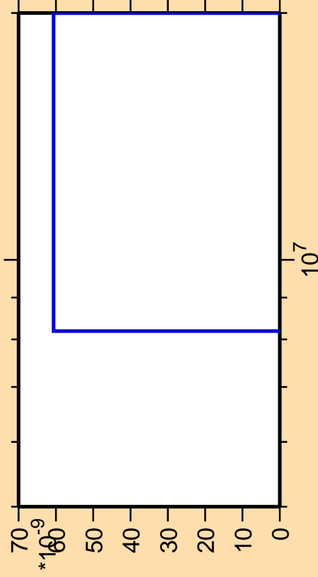
\Delta\sigma/\sigma vs. E for ^{228}\text{Rn} (mt 42)
