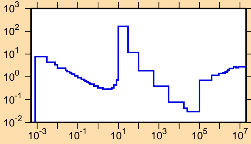
\sigma vs. E for ^{228}\text{Rn}(n,\text{nonel.})
