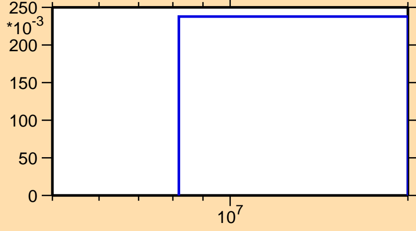
\sigma vs. E for ^{228}\text{Rn}(n,3n)
