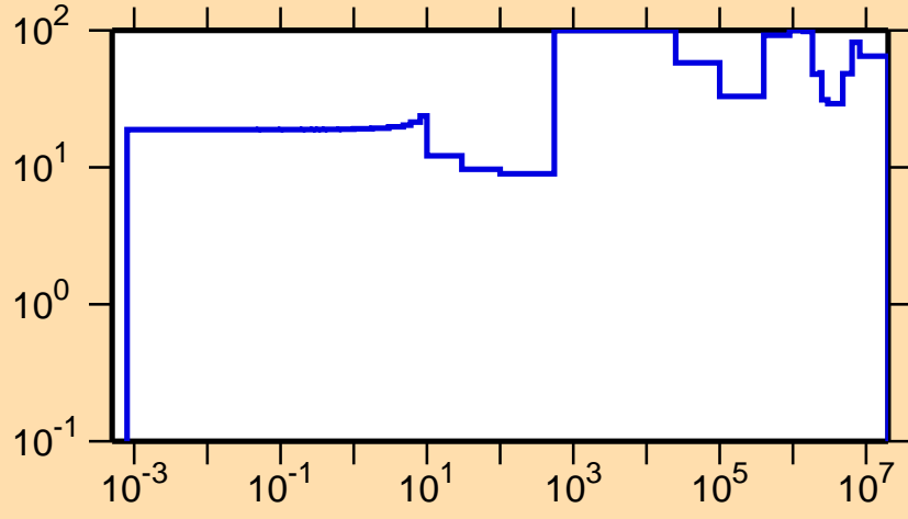
\Delta\sigma/\sigma vs. E for ^{228}\text{Rn}(n,el.)
