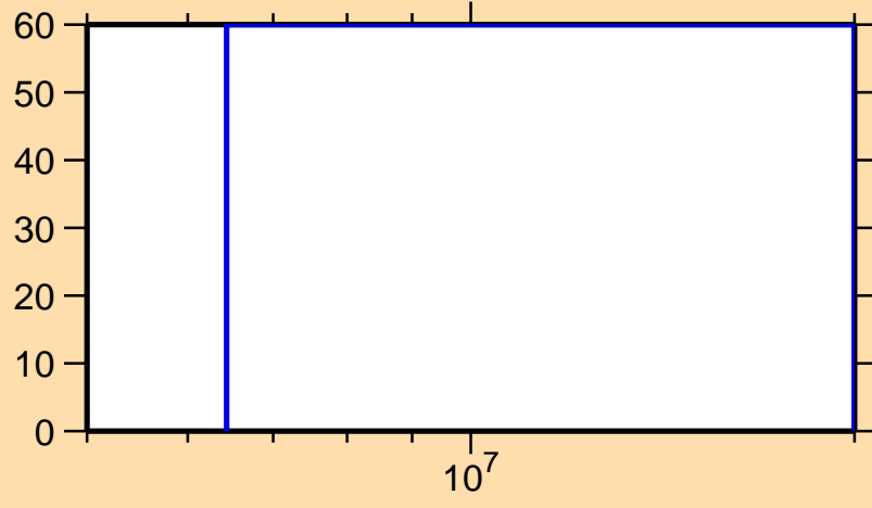
\Delta\sigma/\sigma vs. E for ^{228}\text{Rn}(n,n\text{cont.})
