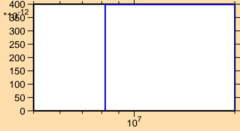
\sigma vs. E for ^{228}\text{Rn}(n,nd)
