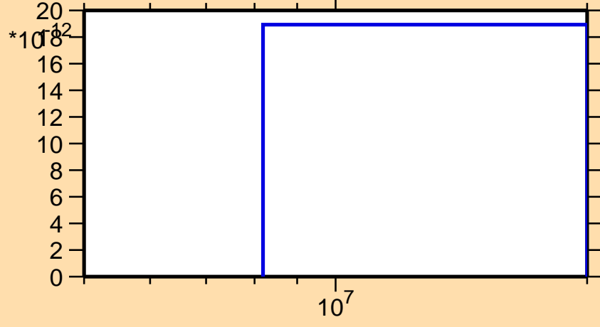
\sigma vs. E for ^{228}\text{Rn}(n,2np)
