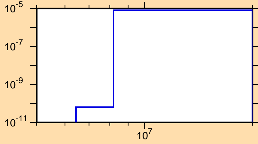
\sigma vs. E for ^{228}\text{Rn}(n,\alpha)
