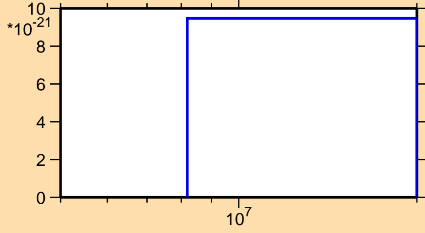
\sigma vs. E for ^{228}\text{Rn} (mt 42)
