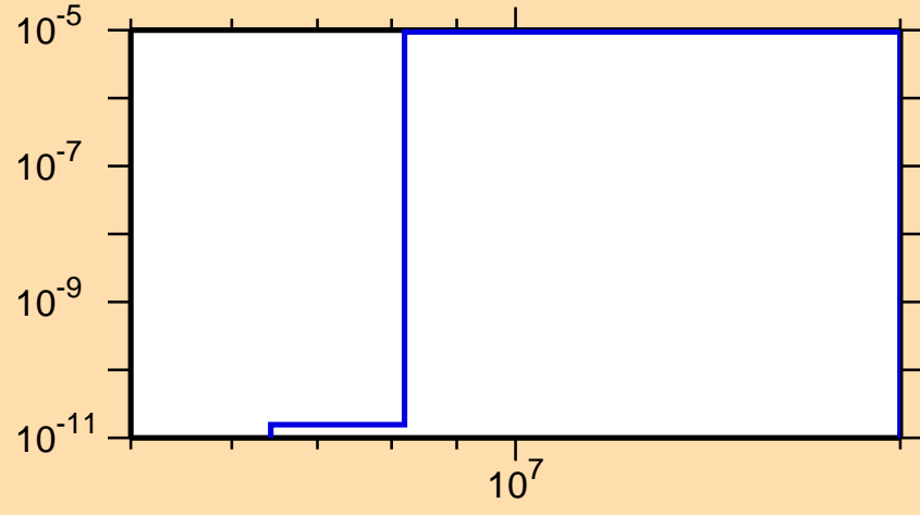
\sigma vs. E for ^{228}\text{Rn}(n,n\alpha)
