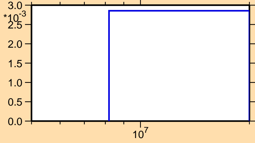
\sigma vs. E for ^{228}\text{Rn}(n,t)
