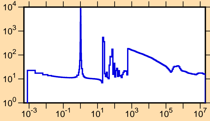
\sigma vs. E for ^{229}\text{Rn}(n,\text{tot.})
