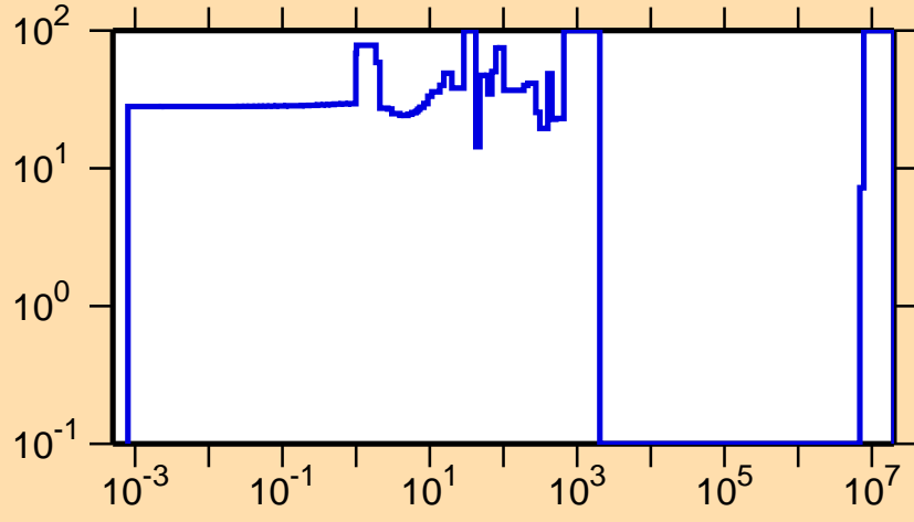
\Delta\sigma/\sigma vs. E for ^{229}\text{Rn}(n,f)
