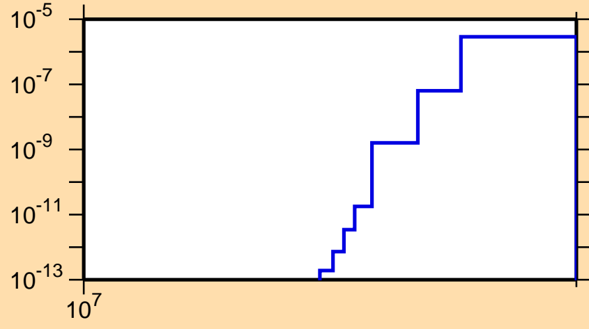
\sigma vs. E for ^{229}\text{Rn}(n,nt)
