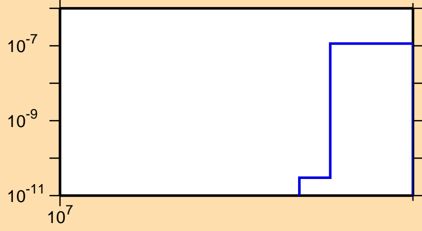
\sigma vs. E for ^{229}\text{Rn}(n,2np)
