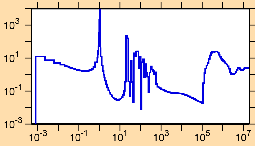
\sigma vs. E for ^{229}\text{Rn}(n,\text{nonel.})
