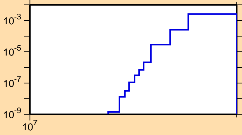
\sigma vs. E for ^{229}\text{Rn}(n,np)
