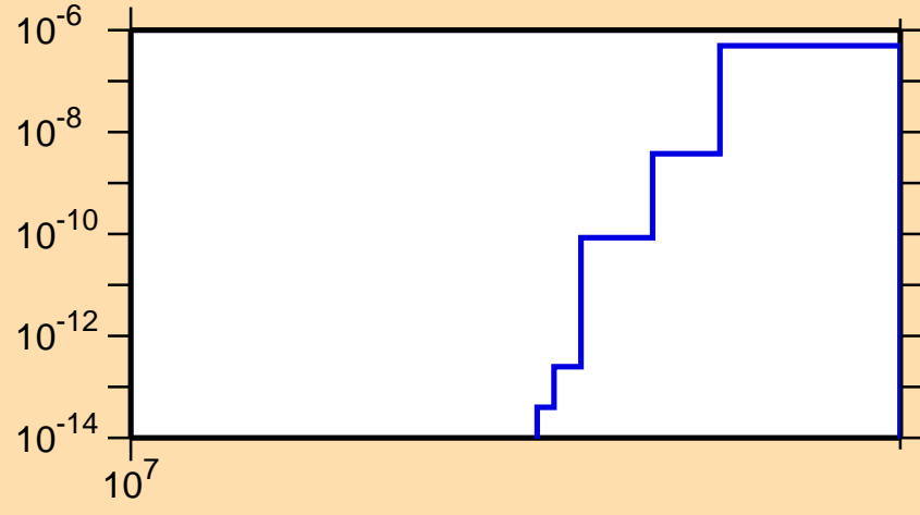
\sigma vs. E for ^{229}\text{Rn}(n,nd)
