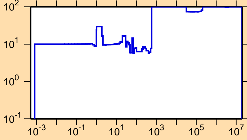
\Delta\sigma/\sigma vs. E for ^{229}\text{Rn}(n,el.)
