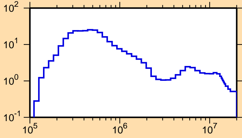
\sigma vs. E for ^{229}\text{Rn}(n,\text{inel.})
