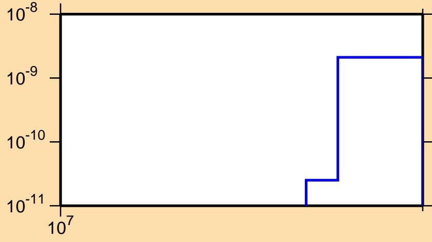
\sigma vs. E for ^{229}\text{Rn}(n,3n\alpha)
