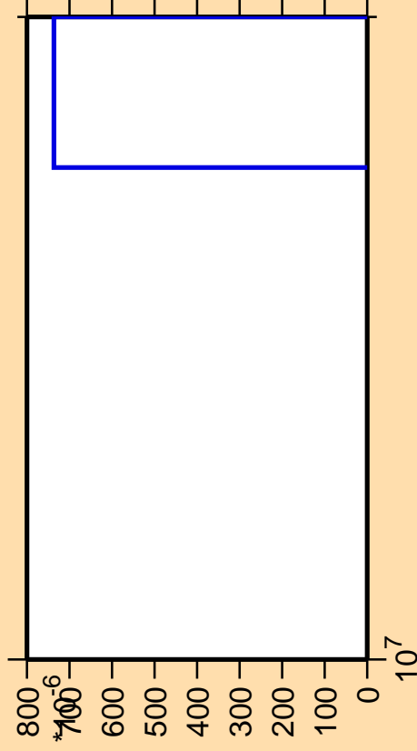
\Delta\sigma/\sigma vs. E for ^{229}\text{Rn} (mt 42)
