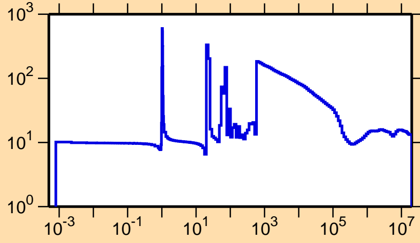
\sigma vs. E for ^{229}\text{Rn}(n,\text{el.})
