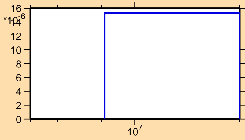
\sigma vs. E for ^{229}\text{Rn}(n,t)
