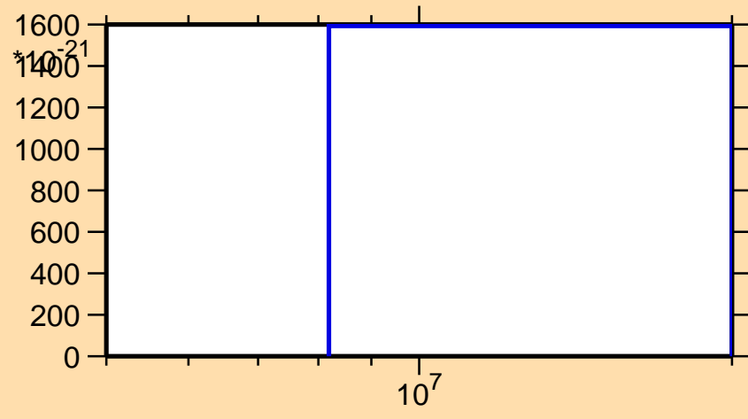
\sigma vs. E for ^{229}\text{Rn} (mt 42)
