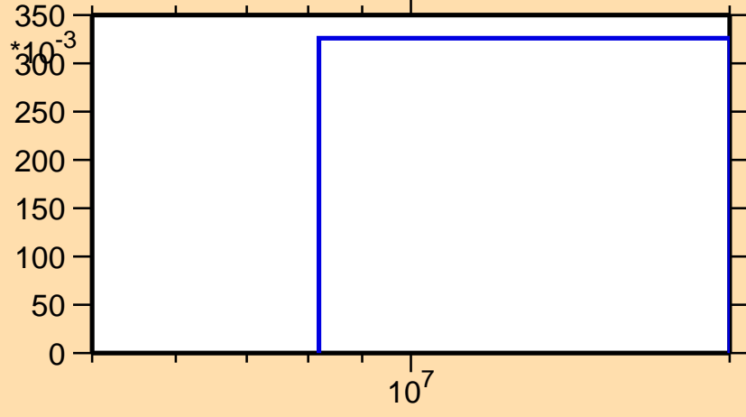
\sigma vs. E for ^{229}\text{Rn}(n,3n)
