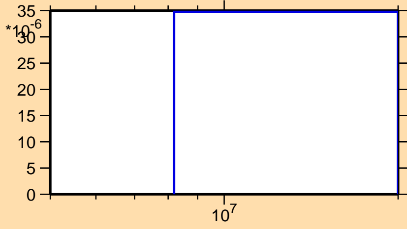
\sigma vs. E for ^{229}\text{Rn}(n,np)
