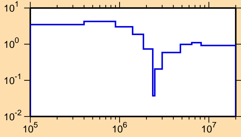
\sigma vs. E for ^{229}\text{Rn}(n,n\text{cont.})
