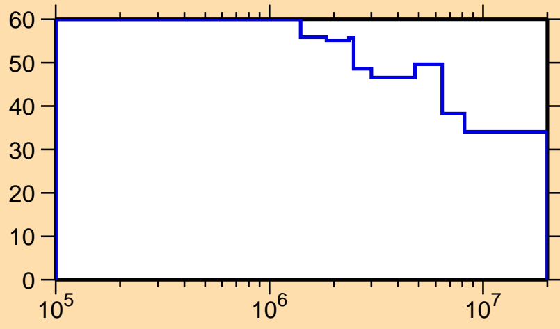
\Delta\sigma/\sigma vs. E for ^{229}\text{Rn}(n,\text{nonel.})
