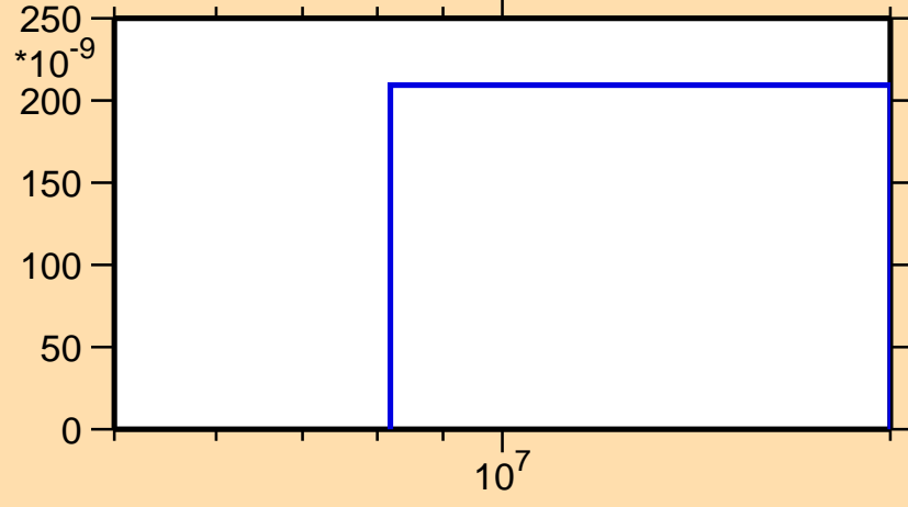
\sigma vs. E for ^{229}\text{Rn}(n,2n\alpha)
