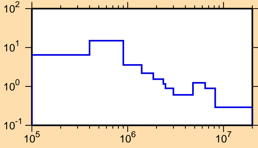
\sigma vs. E for ^{229}\text{Rn}(n,n_1)
