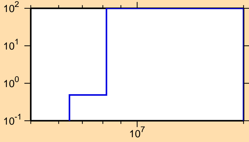
\Delta\sigma/\sigma vs. E for ^{229}\text{Rn}(n,p)
