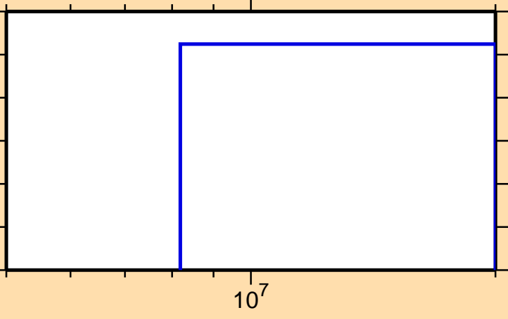
\sigma vs. E for ^{229}\text{Rn}(n,nt)
