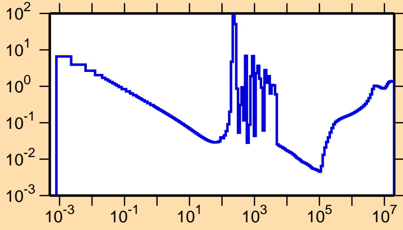
\sigma vs. E for ^{230}\text{Rn}(n,\text{nonel.})
