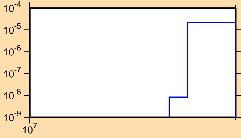
\sigma vs. E for ^{230}\text{Rn}(n,2np)
