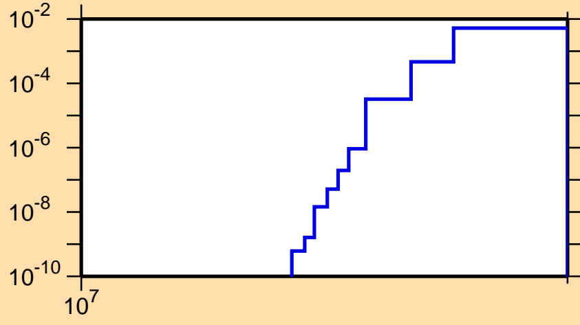
\sigma vs. E for ^{230}\text{Rn}(n,nt)
