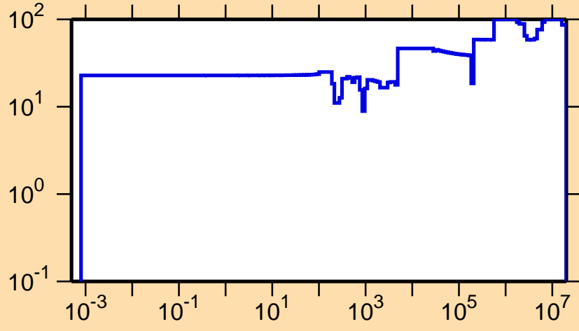
\Delta\sigma/\sigma vs. E for ^{230}\text{Rn}(n,el.)
