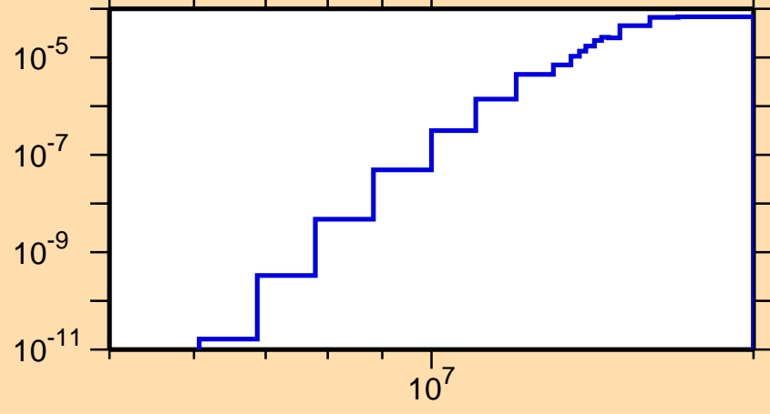
\sigma vs. E for ^{230}\text{Rn}(n,\alpha)
