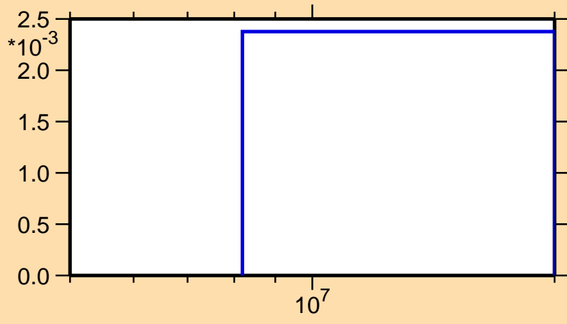
\sigma vs. E for ^{230}\text{Rn}(n,t)
