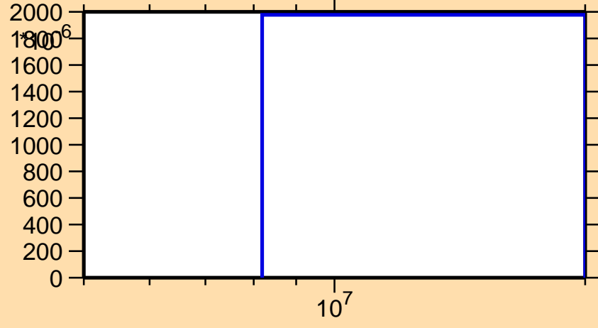
\sigma vs. E for ^{230}\text{Rn}(n,n\alpha)
