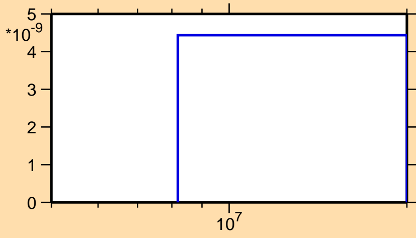
\sigma vs. E for ^{230}\text{Rn}(n,\text{nd})
