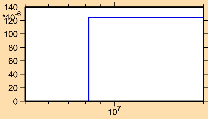
\sigma vs. E for ^{230}\text{Rn}(n,np)
