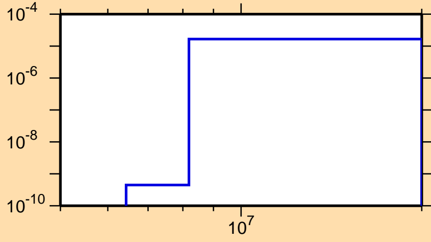
\sigma vs. E for ^{230}\text{Rn}(n,\alpha)
