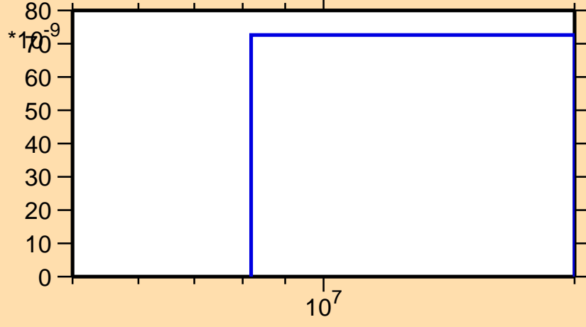
\sigma vs. E for ^{230}\text{Rn}(n,3n)
