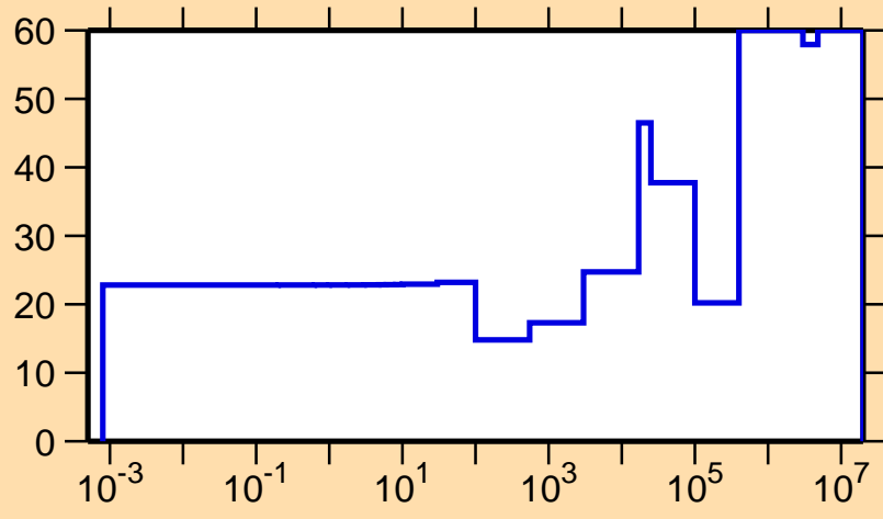
\Delta\sigma/\sigma vs. E for ^{230}\text{Rn}(n,el.)
