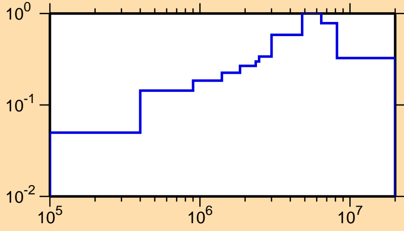
\sigma vs. E for ^{230}\text{Rn}(n,\text{inel.})
