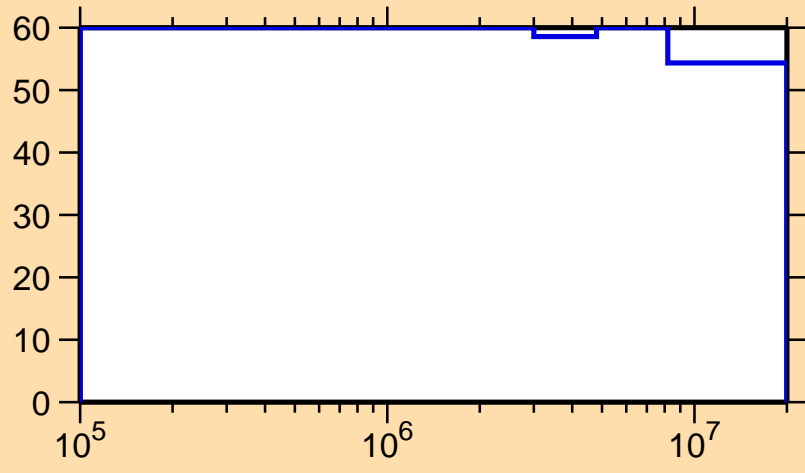
\Delta\sigma/\sigma vs. E for ^{230}\text{Rn}(n,\text{nonel.})
