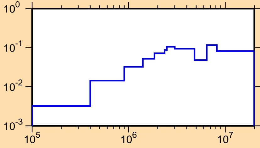
\sigma vs. E for ^{230}\text{Rn}(n,n\text{cont.})
