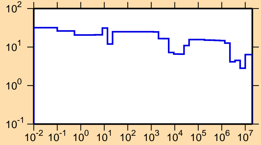
\Delta\sigma/\sigma vs. E for ^{88}\text{Ru}(n,\text{tot.})
