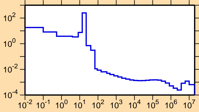
\sigma vs. E for ^{88}\text{Ru}(n,\gamma)
