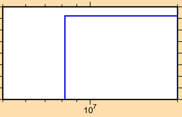
\sigma vs. E for ^{88}\text{Ru}(n,2n)
