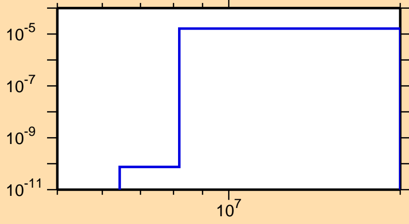
\sigma vs. E for ^{88}\text{Ru}(n,n\alpha)
