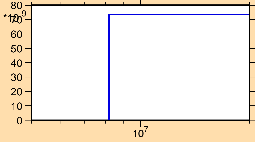
\sigma vs. E for ^{88}\text{Ru}(n,\text{pt})
