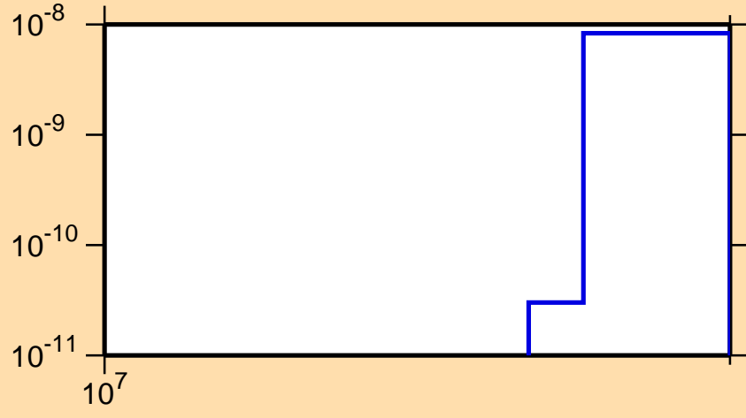
\sigma vs. E for ^{89}\text{Ru}(n,\text{nd})
