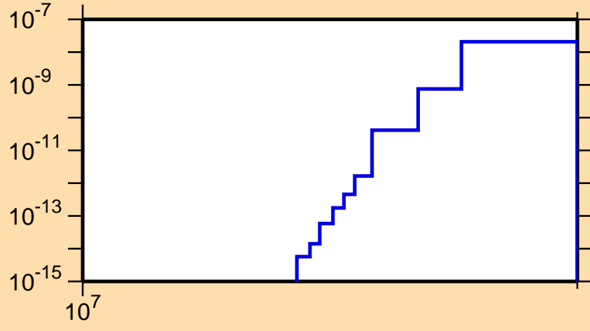
\sigma vs. E for ^{89}\text{Ru} (mt 34)
