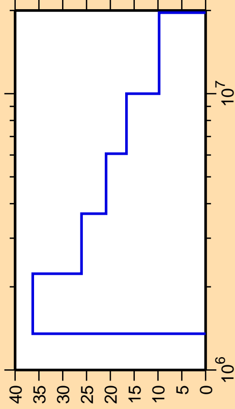
\Delta\sigma/\sigma vs. E for ^{89}\text{Ru}(n,n_4)
