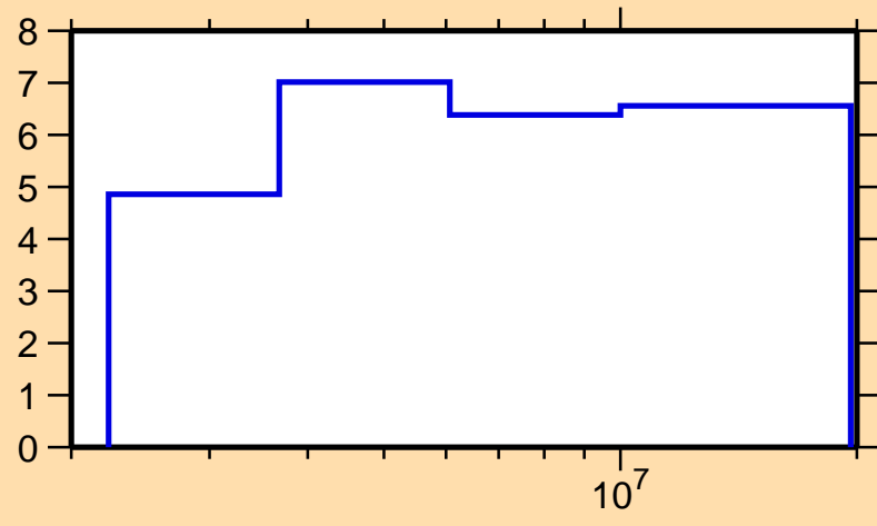
\Delta\sigma/\sigma vs. E for ^{89}\text{Ru}(n,n\text{nonel.})
