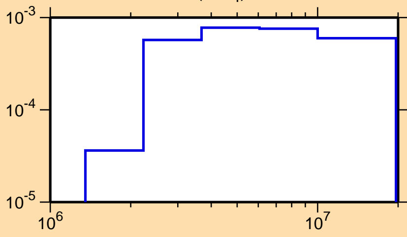
\sigma vs. E for ^{89}\text{Ru}(n,n_4)
