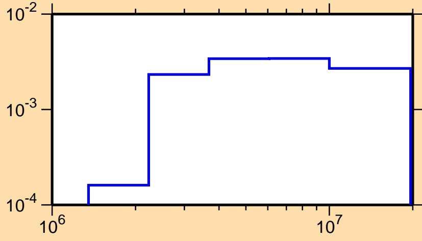
\sigma vs. E for ^{89}\text{Ru}(n,n_3)
