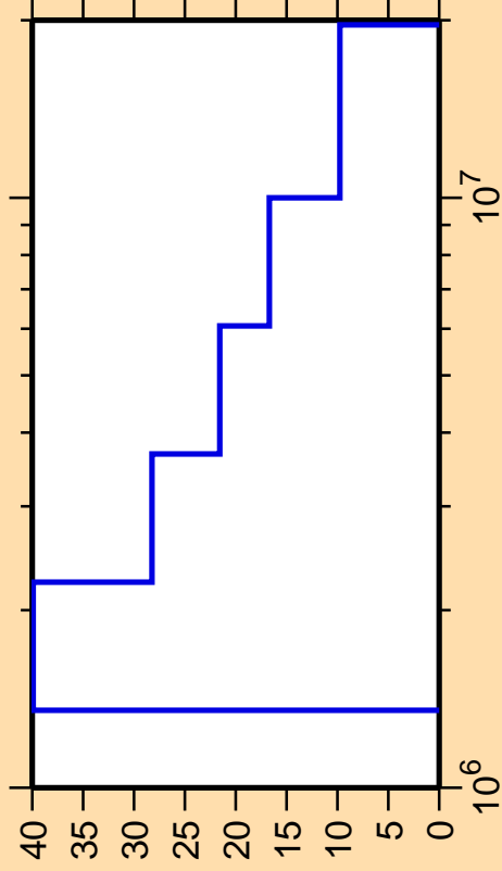
\Delta\sigma/\sigma vs. E for ^{89}\text{Ru}(n,n_3)
