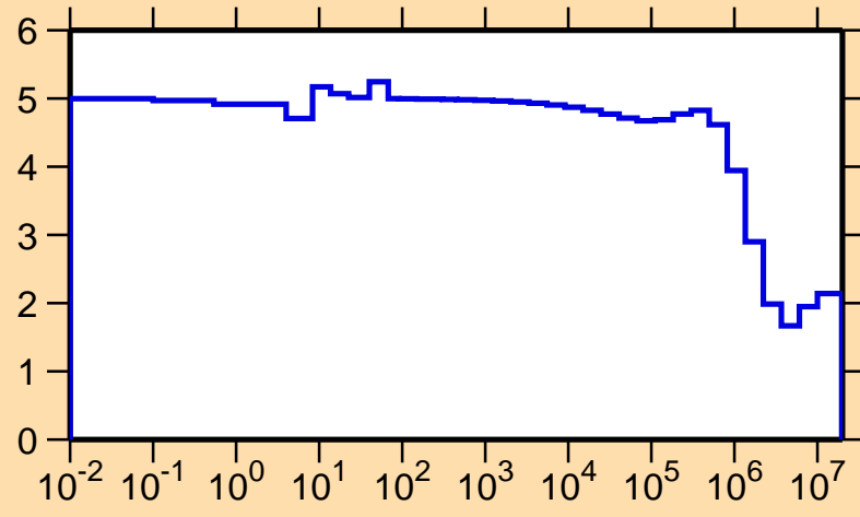
\sigma vs. E for ^{89}\text{Ru}(n,\text{el.})
