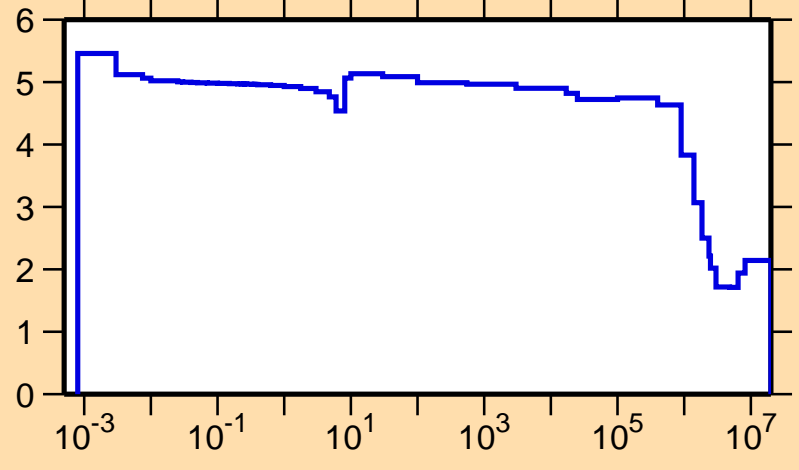
\sigma vs. E for ^{89}\text{Ru}(n,\text{el.})
