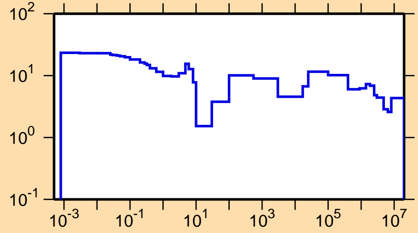
\Delta\sigma/\sigma vs. E for ^{89}\text{Ru}(n,\text{tot.})
