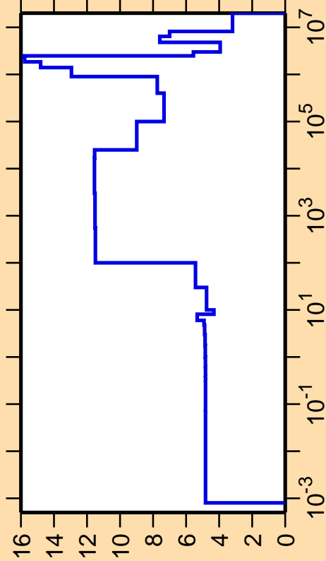
\Delta\sigma/\sigma vs. E for ^{89}\text{Ru}(n,\text{el.})
