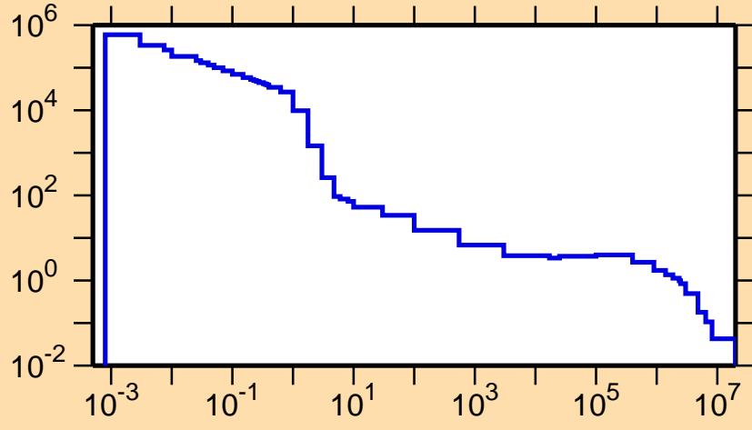
\sigma vs. E for ^{89}\text{Ru}(n,p)
