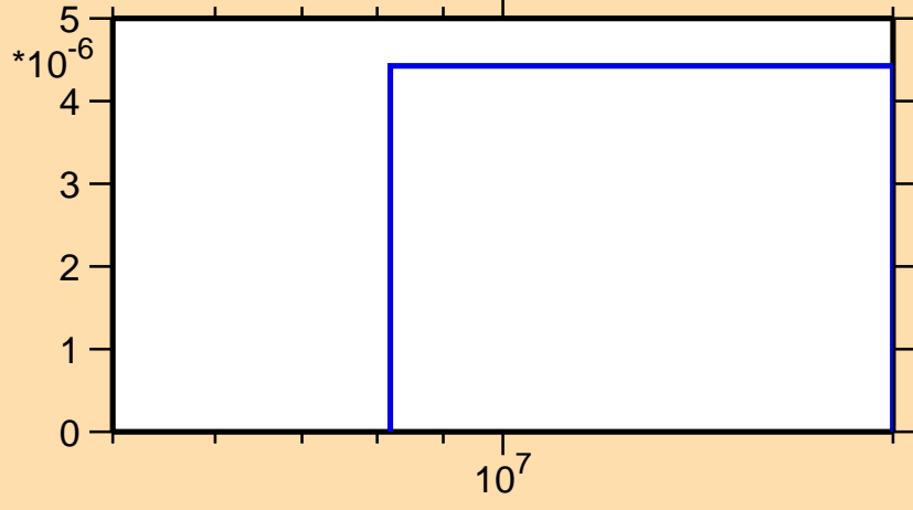
\sigma vs. E for ^{89}\text{Ru}(n,\text{pt})
