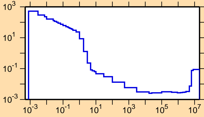
\sigma vs. E for ^{89}\text{Ru}(n,\alpha)
