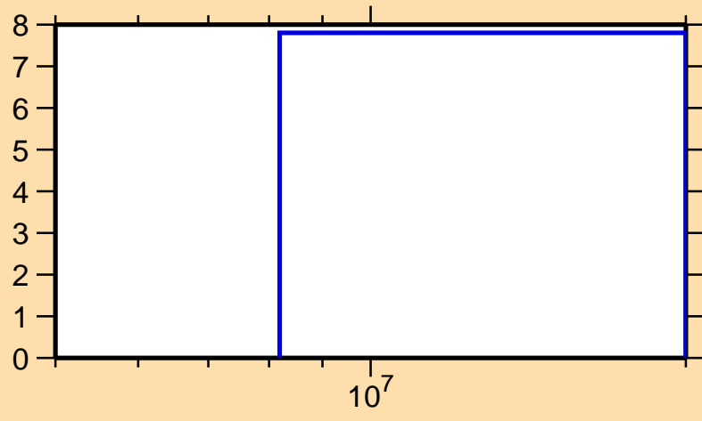
\Delta\sigma/\sigma vs. E for ^{90}\text{Ru}(n,\text{el.})
