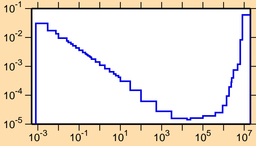
\sigma vs. E for ^{90}\text{Ru}(n,\alpha)
