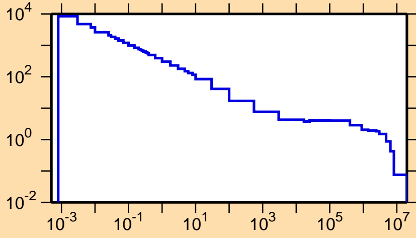
\sigma vs. E for ^{90}\text{Ru}(n,p)
