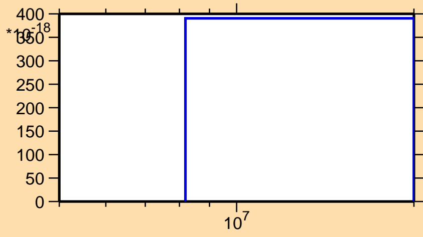
\sigma vs. E for ^{90}\text{Ru}(n,2np)
