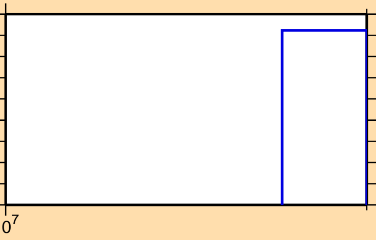
\sigma vs. E for ^{91}\text{Ru}(n,2np)
