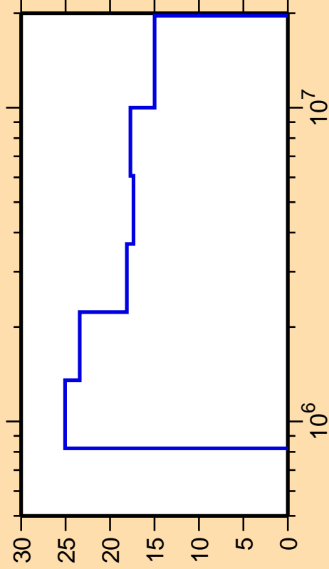
\Delta\sigma/\sigma vs. E for ^{91}\text{Ru}(n,n_4)
