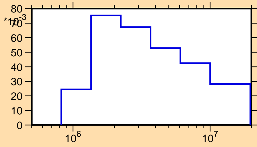
\sigma vs. E for ^{91}\text{Ru}(n,n_4)
