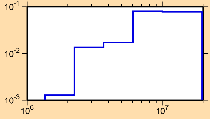
\sigma vs. E for ^{91}\text{Ru}(n,n\text{cont.})
