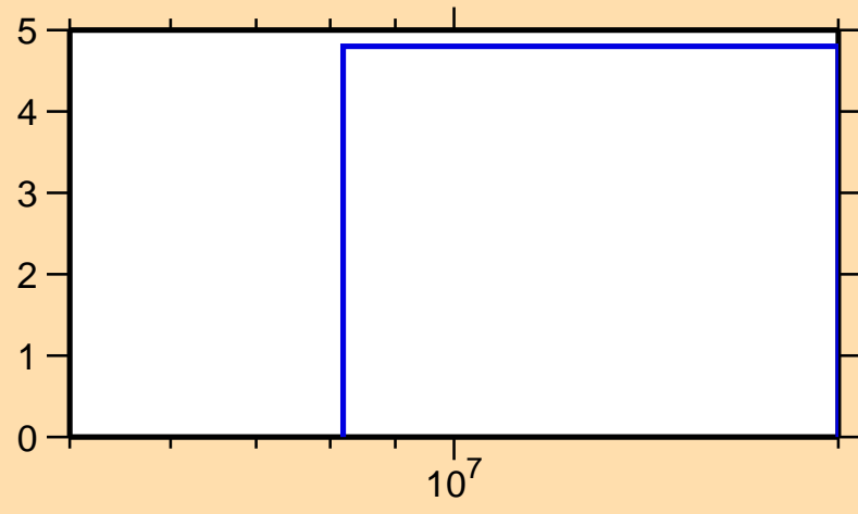
\Delta\sigma/\sigma vs. E for ^{91}\text{Ru}(n,\text{el.})
