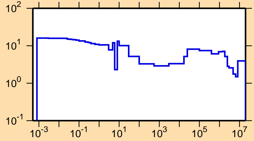
\Delta\sigma/\sigma vs. E for ^{91}\text{Ru}(n,\text{tot.})
