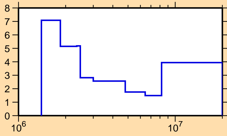
\Delta\sigma/\sigma vs. E for ^{91}\text{Ru}(n,\text{tot.})
