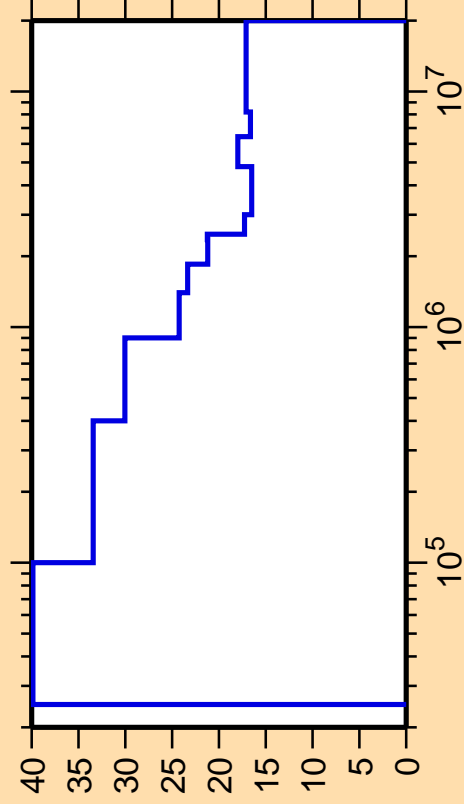
\Delta\sigma/\sigma vs. E for ^{91}\text{Ru}(n,\text{inel.})
