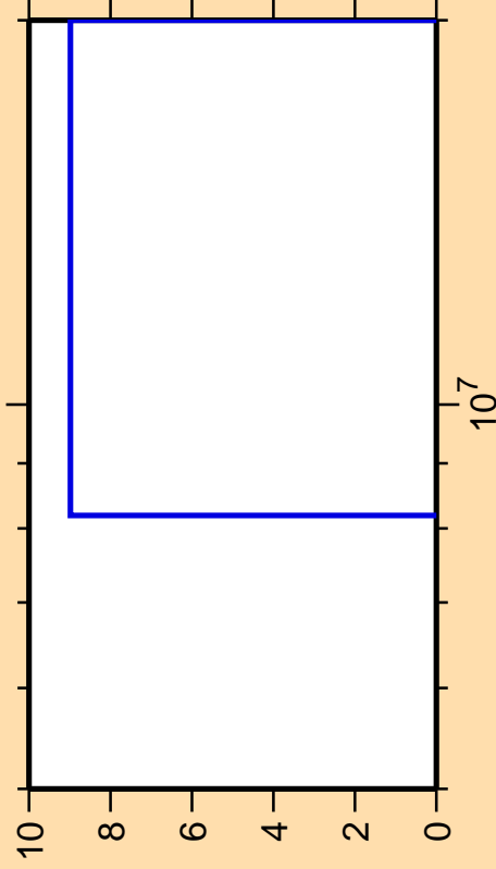
\Delta\sigma/\sigma vs. E for ^{91}\text{Ru}(\text{mt } 45)
