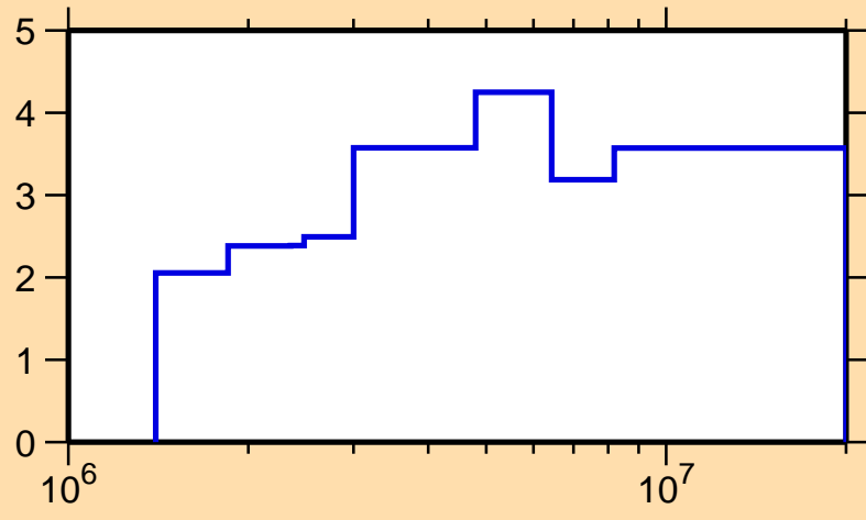
\Delta\sigma/\sigma vs. E for ^{91}\text{Ru}(n,\text{nonel.})
