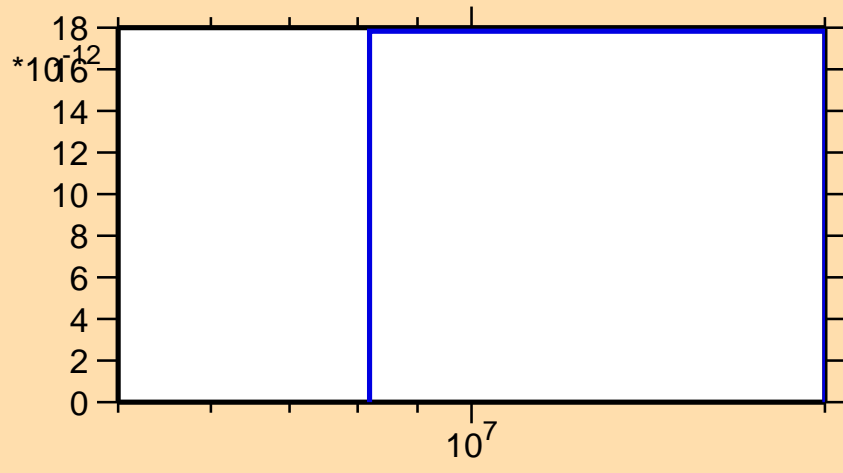
\sigma vs. E for ^{91}\text{Ru}(\text{mt } 45)
