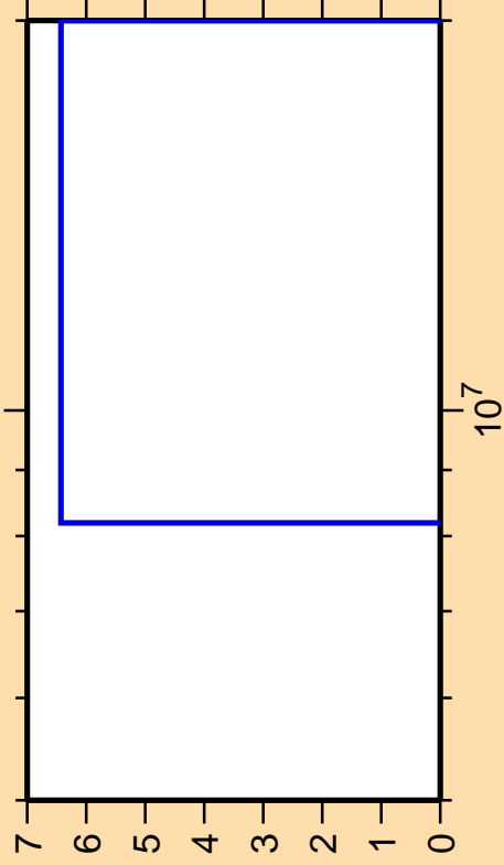
\Delta\sigma/\sigma vs. E for ^{91}\text{Ru}(n,p)
