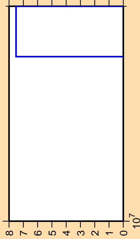
\Delta\sigma/\sigma vs. E for ^{92}\text{Ru}(n,\text{nd})
