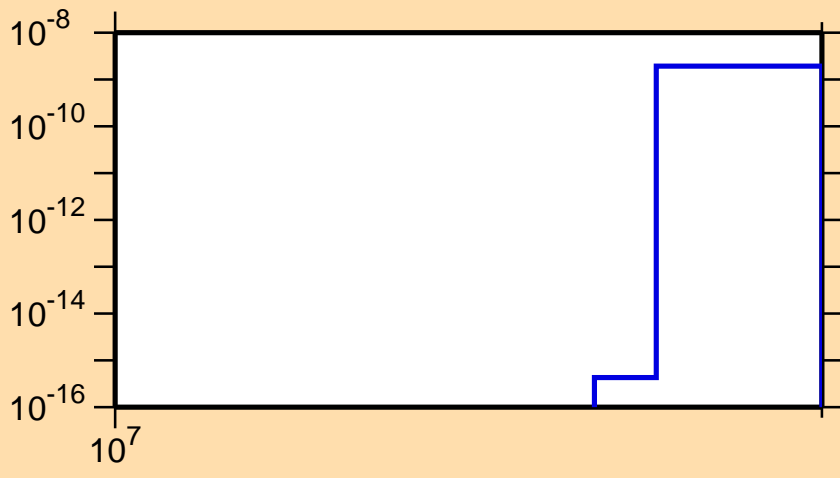
\sigma vs. E for ^{92}\text{Ru}(n,\text{pt})
