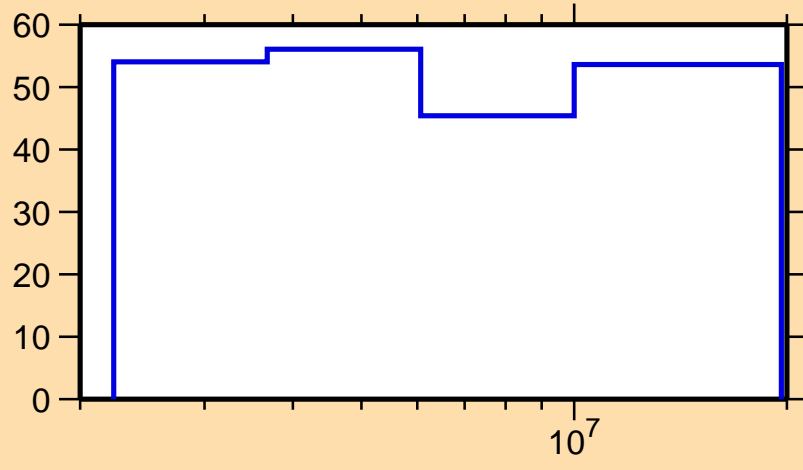
\Delta\sigma/\sigma vs. E for ^{92}\text{Ru}(n,ncont.)
