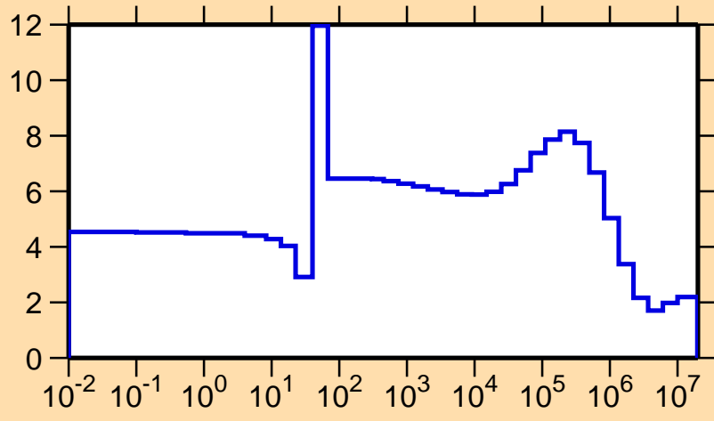
\sigma vs. E for ^{92}\text{Ru}(n,\text{el.})
