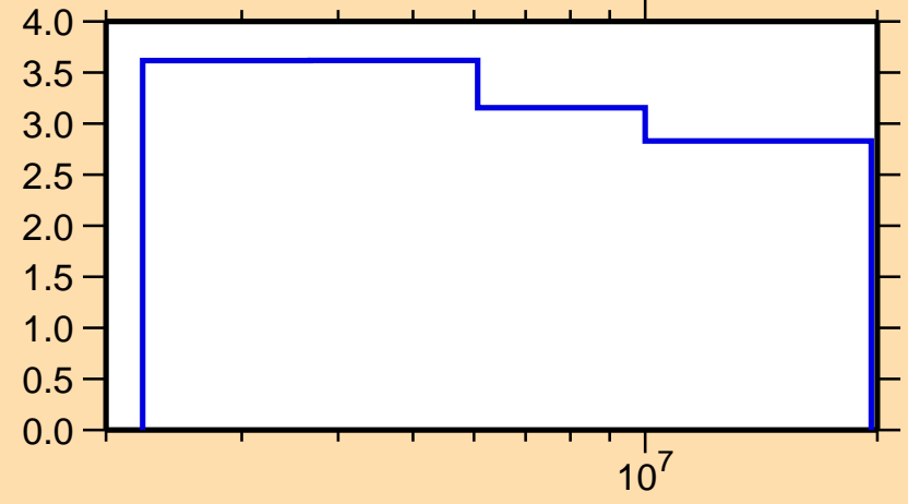
\Delta\sigma/\sigma vs. E for ^{92}\text{Ru}(n,n\text{nonel.})
