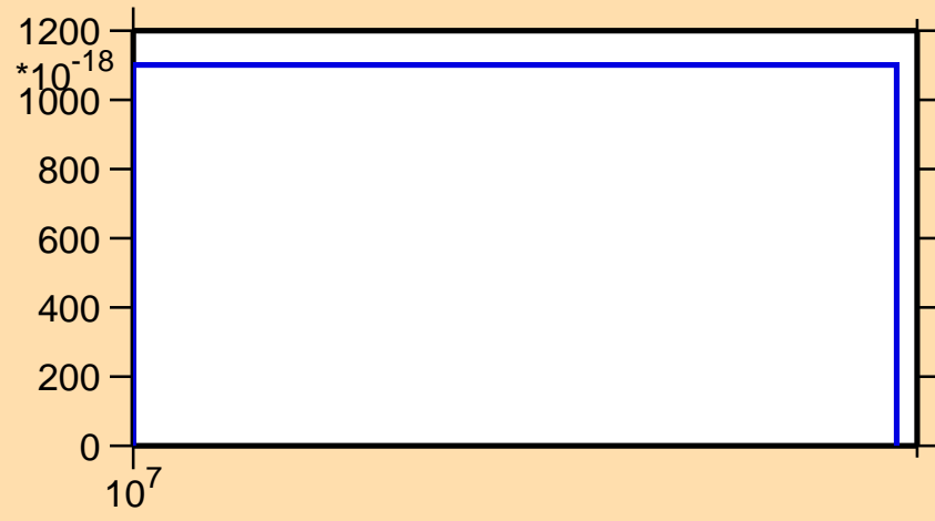
\sigma vs. E for ^{92}\text{Ru}(\text{mt } 34)
