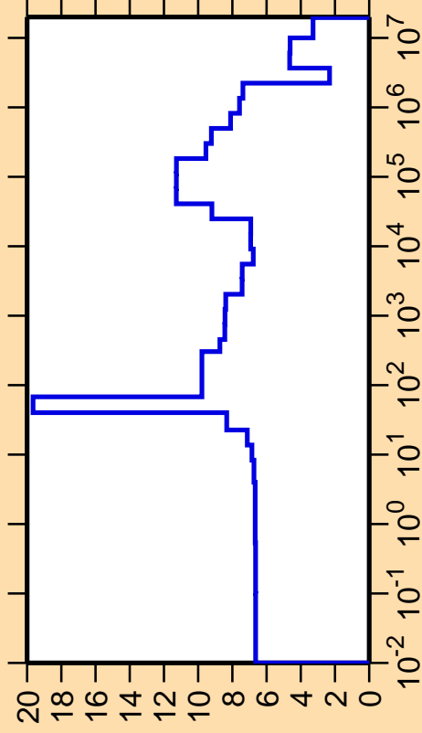
\Delta\sigma/\sigma vs. E for ^{92}\text{Ru}(n,\text{el.})
