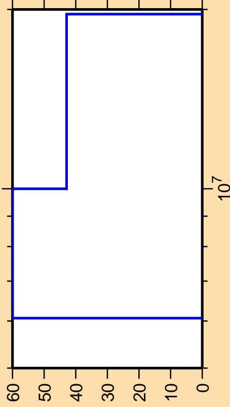
\Delta\sigma/\sigma vs. E for ^{92}\text{Ru}(n,n\alpha)
