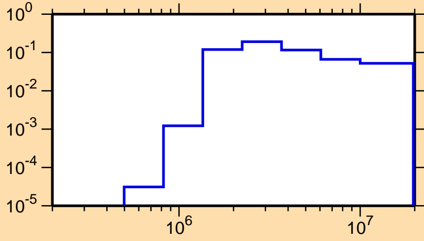
\sigma vs. E for ^{93}\text{Ru}(n,\text{inel.})
