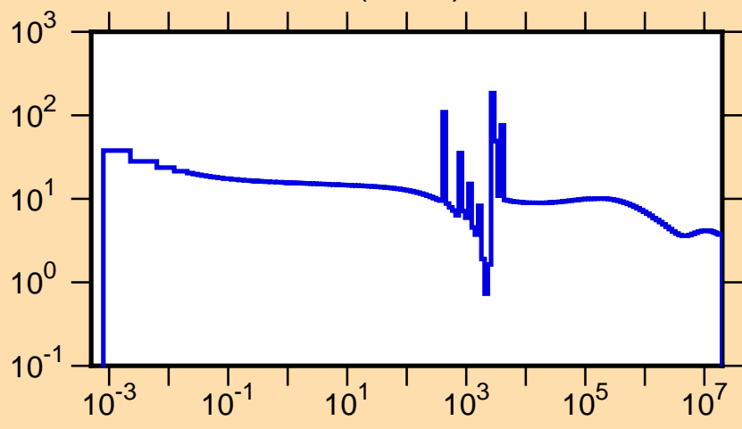
\sigma vs. E for ^{94}\text{Ru}(n,\text{tot.})
