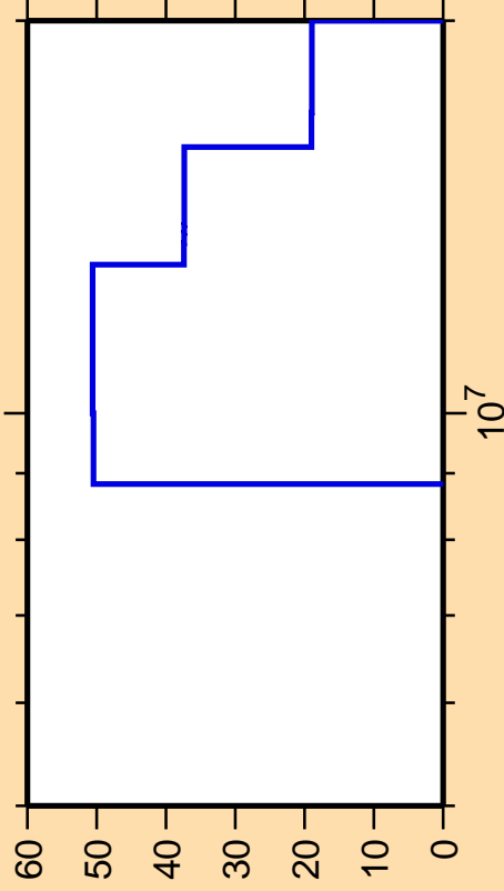
\Delta\sigma/\sigma vs. E for ^{94}\text{Ru}(n,n\alpha)
