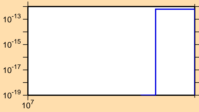
\sigma vs. E for ^{94}\text{Ru} (mt 45)
