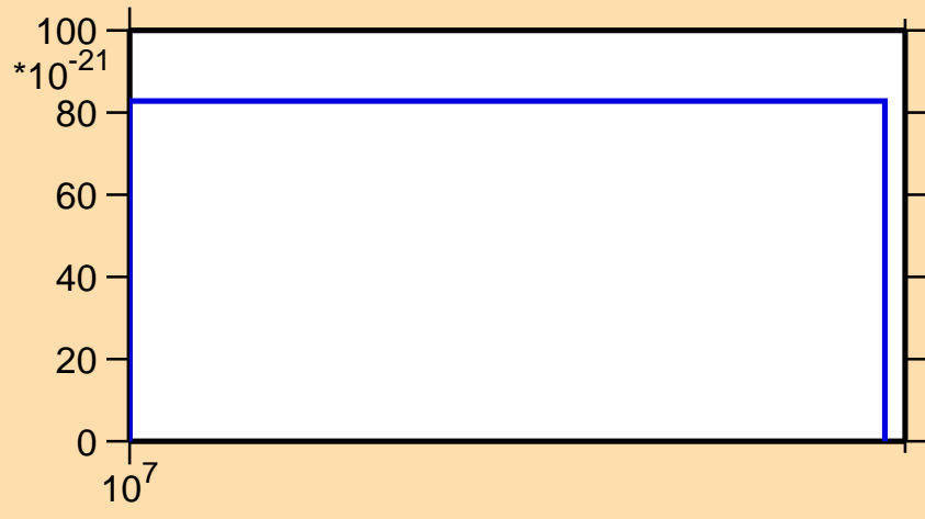
\sigma vs. E for ^{94}\text{Ru}(n,2np)
