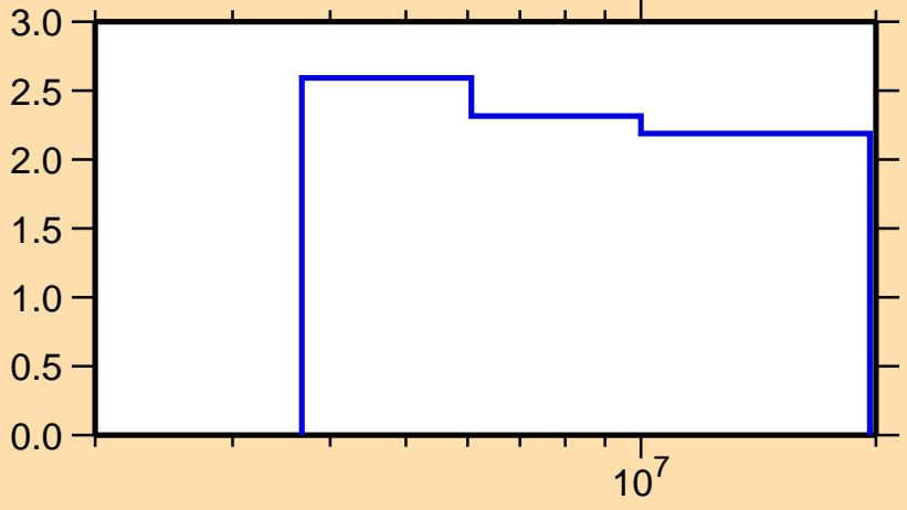
\Delta\sigma/\sigma vs. E for ^{94}\text{Ru}(n,n\text{nonel.})
