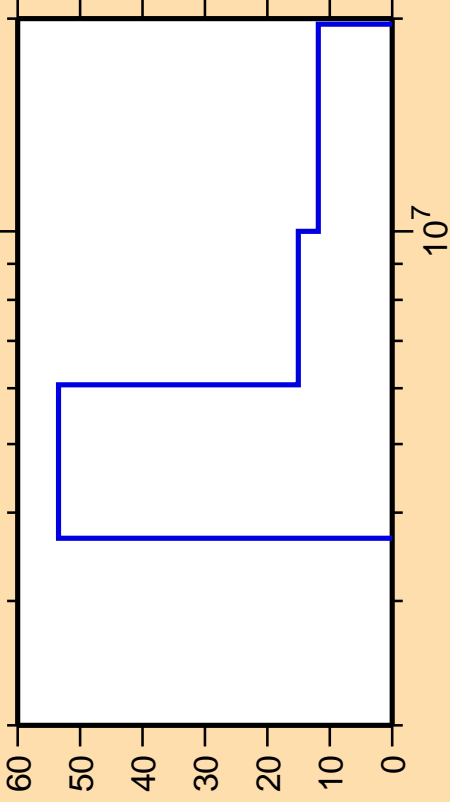
\Delta\sigma/\sigma vs. E for ^{94}\text{Ru}(n,n\text{cont.})
