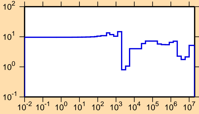
\Delta\sigma/\sigma vs. E for ^{94}\text{Ru}(n,el.)
