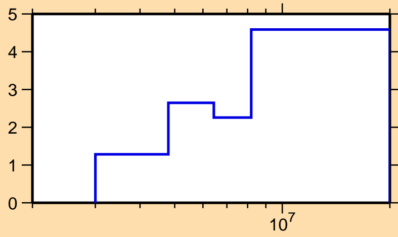
\Delta\sigma/\sigma vs. E for ^{94}\text{Ru}(n,\text{el.})
