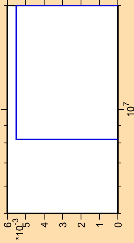
\Delta\sigma/\sigma vs. E for ^{94}\text{Ru} (mt 45)
