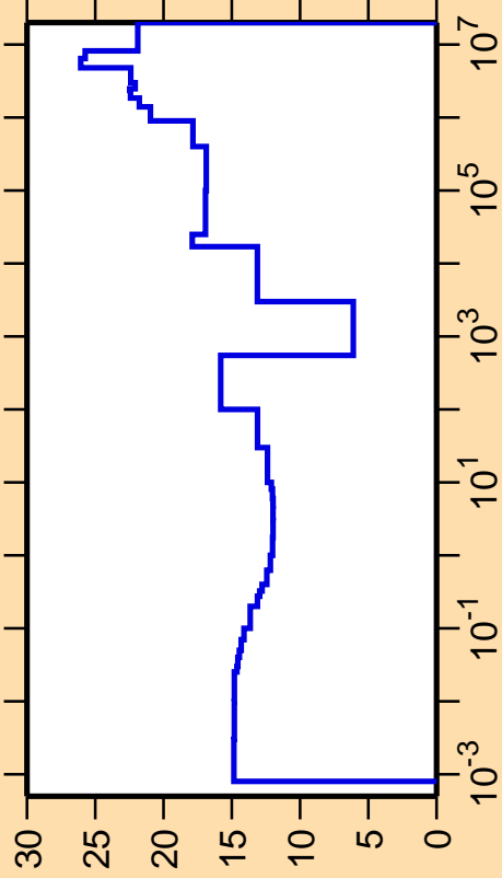
\Delta\sigma/\sigma vs. E for ^{94}\text{Ru}(n,\gamma)
