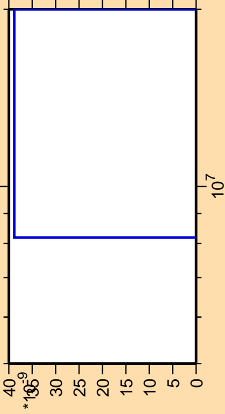
\Delta\sigma/\sigma vs. E for ^{94}\text{Ru}(n,2np)
