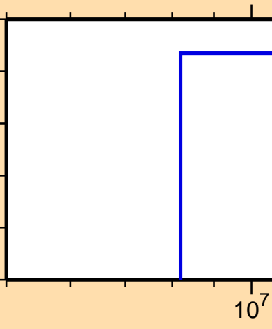
\sigma vs. E for ^{94}\text{Ru}(n,2n\alpha)
