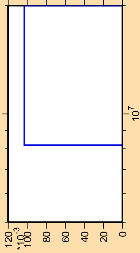
\Delta\sigma/\sigma vs. E for ^{94}\text{Ru}(n,\text{pt})
