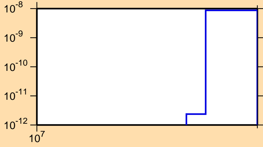
\sigma vs. E for ^{97}\text{Ru}(n,\text{pt})
