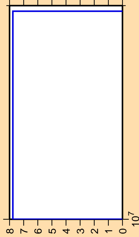
\Delta\sigma/\sigma vs. E for ^{97}\text{Ru} (mt 45)
