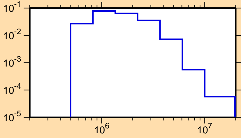
\sigma vs. E for ^{97}\text{Ru}(n,n_4)
