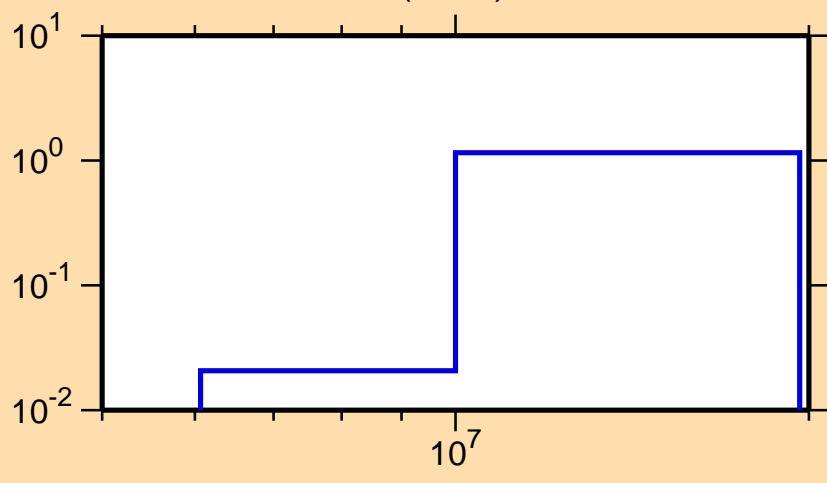
\sigma vs. E for ^{97}\text{Ru}(n,2n)
