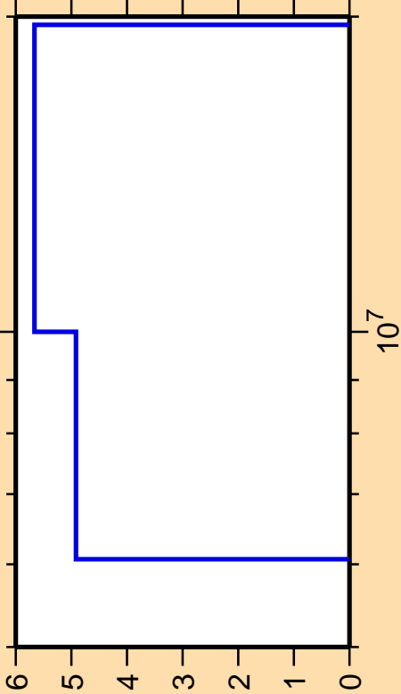
\Delta\sigma/\sigma vs. E for ^{97}\text{Ru}(n,2n)
