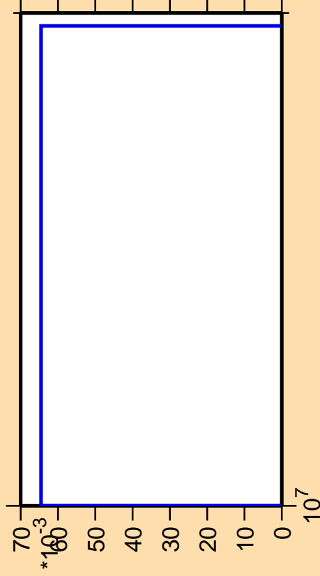
\Delta\sigma/\sigma vs. E for ^{97}\text{Ru}(n,nt)
