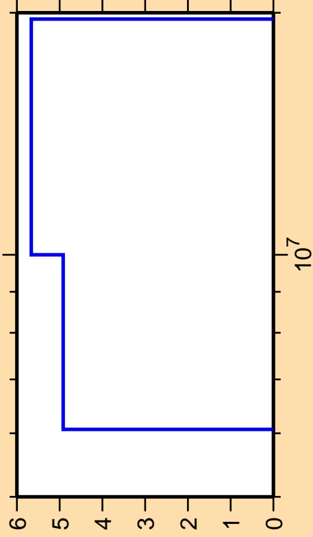
\Delta\sigma/\sigma vs. E for ^{97}\text{Ru}(n,2n)
