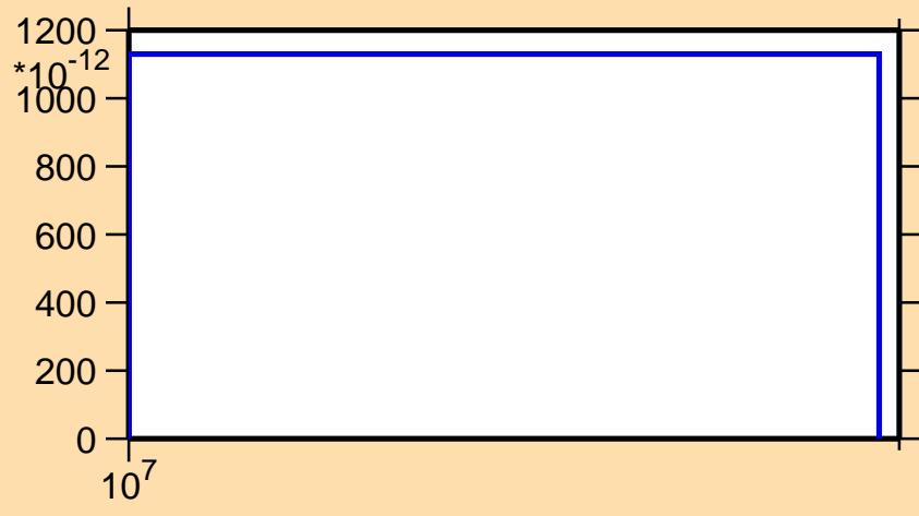
\sigma vs. E for ^{97}\text{Ru}(n,\text{pd})
