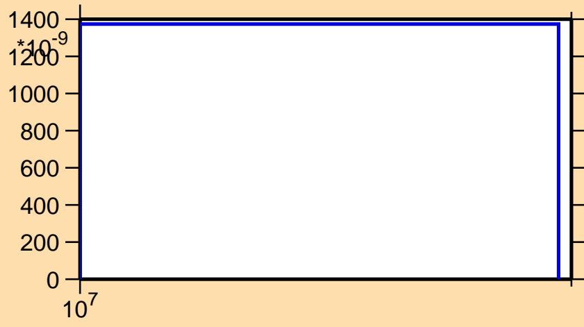
\sigma vs. E for ^{97}\text{Ru}(n,2np)
