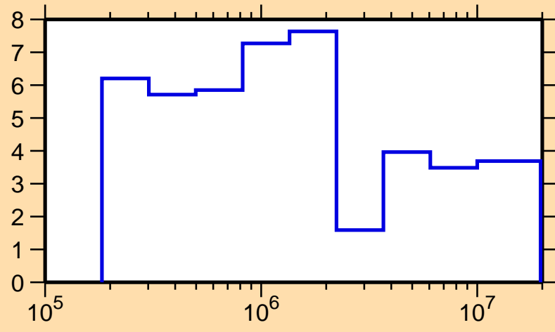
\Delta\sigma/\sigma vs. E for ^{97}\text{Ru}(n,\text{el.})
