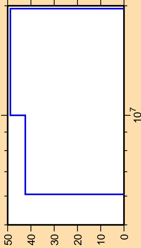
\Delta\sigma/\sigma vs. E for ^{97}\text{Ru}(n,p\alpha)
