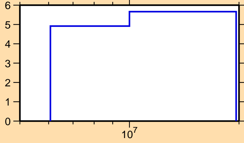
\Delta\sigma/\sigma vs. E for ^{97}\text{Ru}(n,2n)
