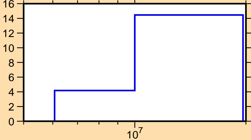
\Delta\sigma/\sigma vs. E for ^{97}\text{Ru}(n,\text{inel.})
